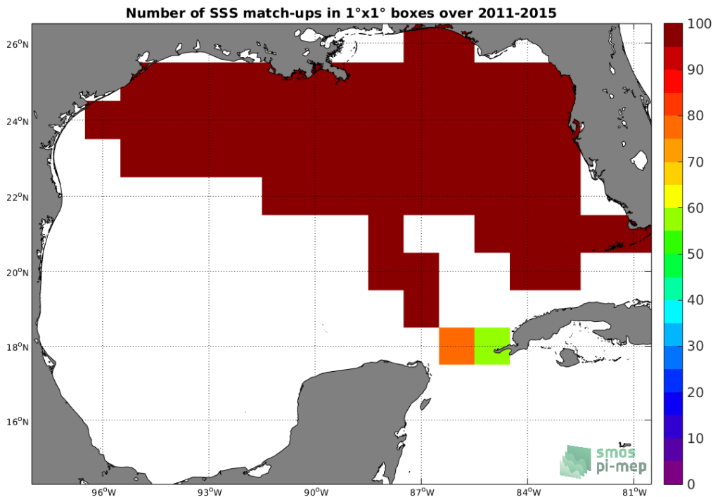
Figure 4: Number of SSS match-ups between TSG-SAMOS SSS and the Aquarius-L3-OR-V5-MONTHLY-RAIN-MASK-1DEG SSS product for the Gulf of Mexico Pi-MEP region over 1°x1° boxes and for the full satellite product period.
