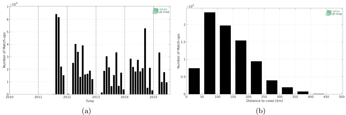
Figure 1: Number of match-ups between TSG-SAMOS and Aquarius-L3-OR-V5-MONTHLY-RAIN-MASK-1DEG SSS as a function of time (a) and as function of the distance to coast (b) over the Gulf of Mexico Pi-MEP region and for the full satellite product period.
