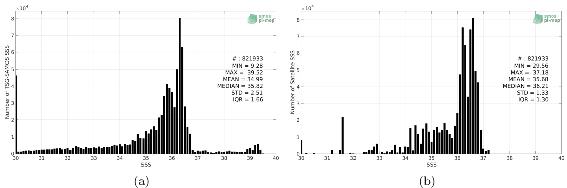
Figure 2: Histograms of SSS from TSG-SAMOS (a) and Aquarius-L3-OR-V5-MONTHLY-RAIN-MASK-1DEG (b) considering all match-up pairs per bins of 0.1 over the Gulf of Mexico Pi-MEP region and for the full satellite product period.
