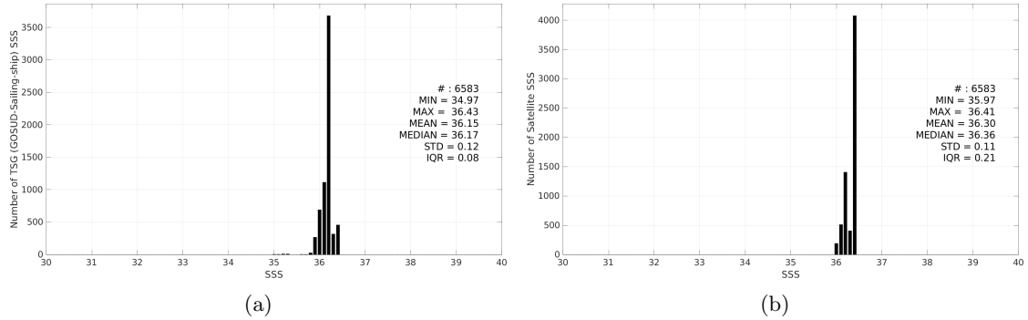
Figure 3: Histograms of SSS from TSG (GOSUD-Sailing-ship) (a) and Aquarius SSS L3 OR v5 - Monthly - Rain mask (NASA-GSFC) (b) considering all match-up pairs per bins of 0.1 over the Gulf of Mexico Pi-MEP region and for the full satellite product period.
