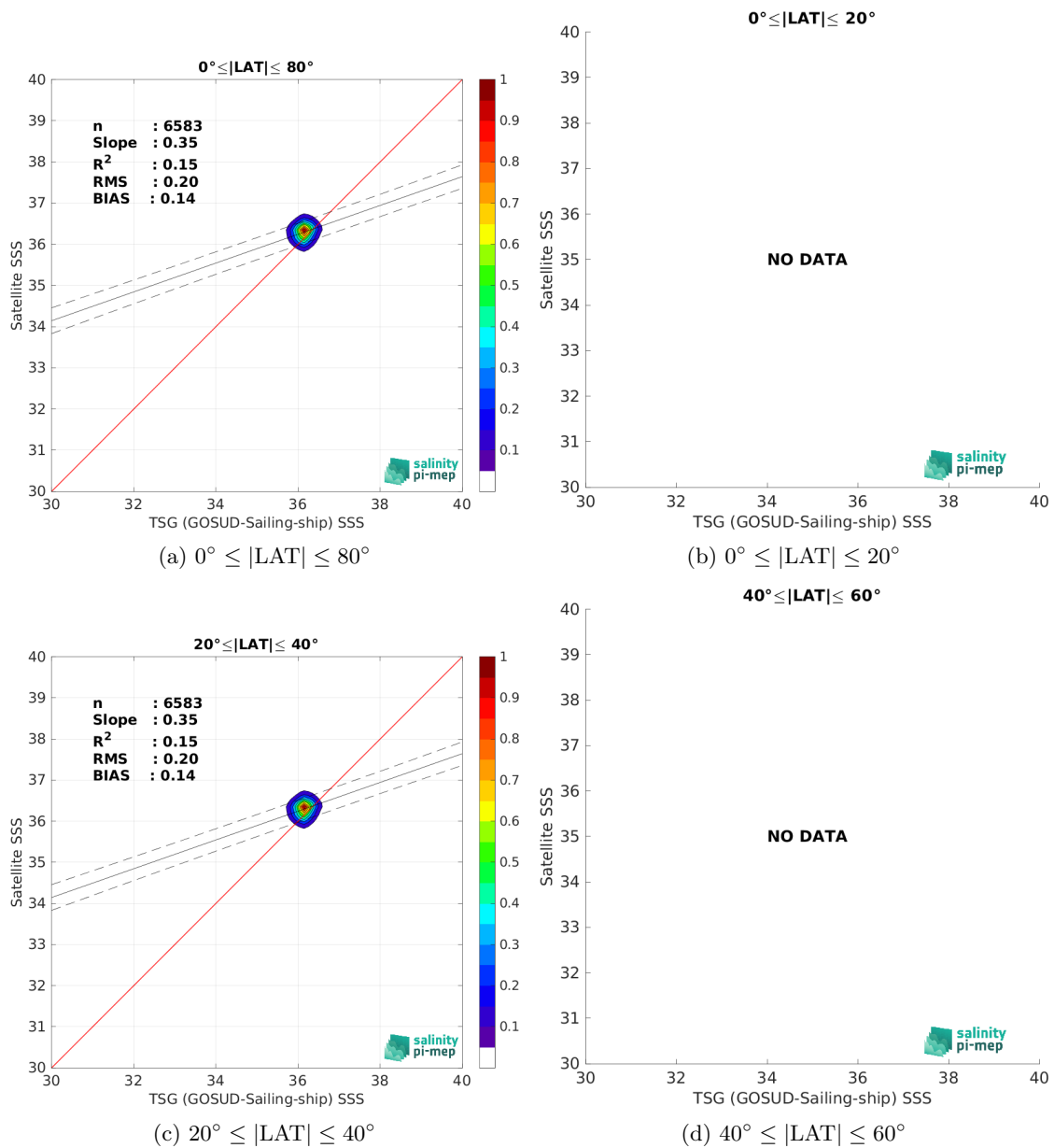
Figure 10: Contour maps of the concentration of Aquarius SSS L3 OR v5 - Monthly - Rain mask (NASA-GSFC) SSS (y-axis) versus TSG (GOSUD-Sailing-ship) SSS (x-axis) at match-up pairs for different latitude bands. For each plot, the red line shows x=y . The black thin and dashed lines indicate a linear fit through the data cloud and the \pm 95\% confidence levels, respectively. The number match-up pairs n , the slope and R^2 coefficient of the linear fit, the root mean square (RMS) and the mean bias between satellite and in situ data are indicated for each latitude band in each plots.
