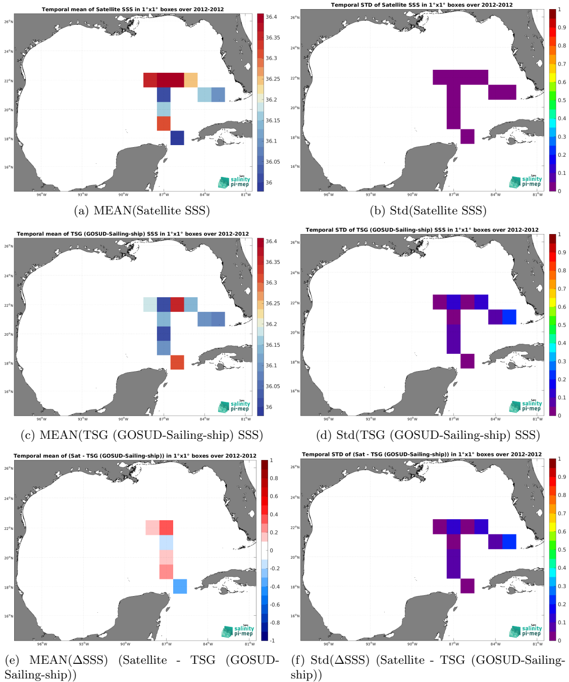
Figure 7: Temporal mean (left) and Std (right) of SSS from Aquarius SSS L3 OR v5 - Monthly - Rain mask (NASA-GSFC) (top), TSG (GOSUD-Sailing-ship) (middle), and of \Delta SSS (Satellite - TSG (GOSUD-Sailing-ship)). Only match-up pairs are used to generate these maps.
