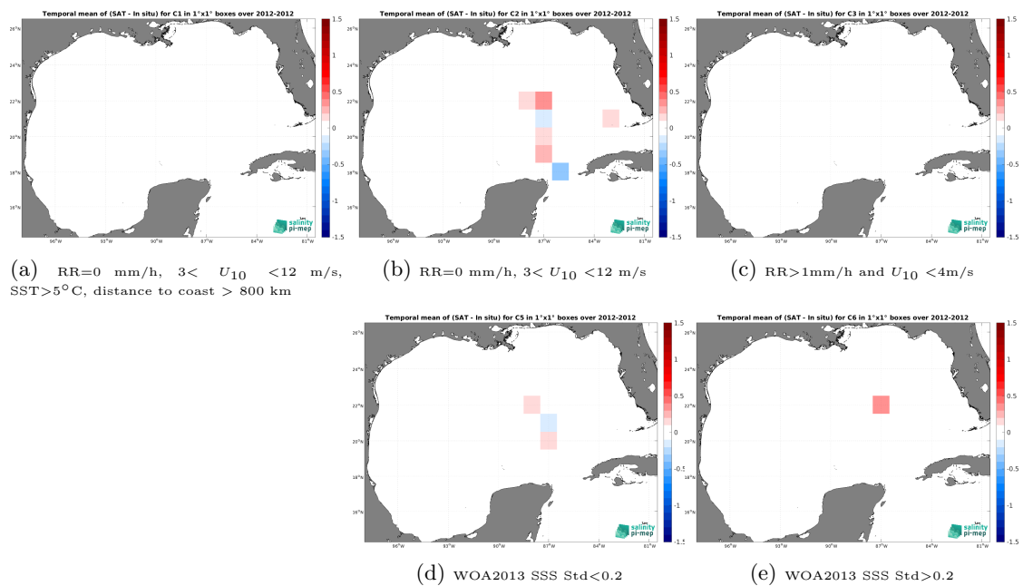
Figure 14: Temporal mean gridded over spatial boxes of size 1^\circ \times 1^\circ of \Delta\text{SSS} (Aquarius SSS L3 OR v5 - Monthly - Rain mask (NASA-GSFC) - TSG (GOSUD-Sailing-ship)) for 5 different subdatasets corresponding to:RR=0 mm/h, 3 < U_{10} < 12 m/s, SST>5°C, distance to coast > 800 km (a), RR=0 mm/h, 3 < U_{10} < 12 m/s (b), RR>1mm/h and U_{10} < 4 m/s (c), WOA2013 SSS Std<0.2 (d), WOA2013 SSS Std>0.2 (e).
