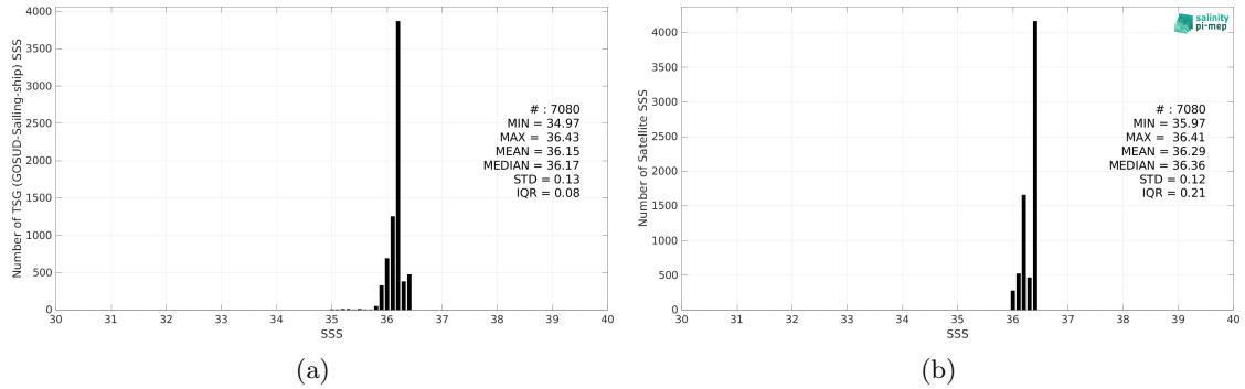
Figure 2: Histograms of SSS from TSG (GOSUD-Sailing-ship) (a) and Aquarius SSS L3 OR v5 - Monthly - Rain mask (NASA-GSFC) (b) considering all match-up pairs per bins of 0.1 over the Gulf of Mexico Pi-MEP region and for the full satellite product period.
