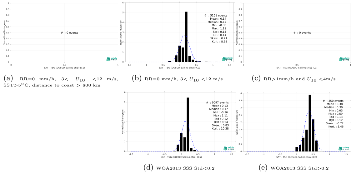
Figure 13: Normalized histogram of \Delta\text{SSS} (Aquarius SSS L3 OR v5 - Monthly - Rain mask (NASA-GSFC) - TSG (GOSUD-Sailing-ship)) for 5 different subdatasets corresponding to: RR=0 mm/h, 3 < U_{10} < 12 m/s, SST > 5^\circ\text{C} , distance to coast > 800 km (a), RR=0 mm/h, 3 < U_{10} < 12 m/s (b), RR > 1\text{mm/h} and U_{10} < 4\text{m/s} (c), WOA2013 SSS Std < 0.2 (d), WOA2013 SSS Std > 0.2 (e).
