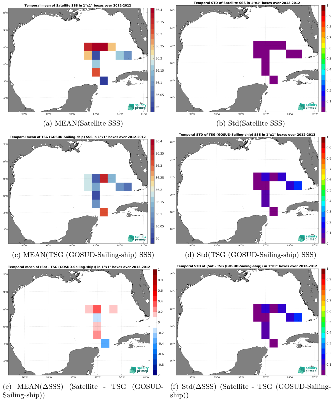
Figure 6: Temporal mean (left) and Std (right) of SSS from Aquarius SSS L3 OR v5 - Monthly - Rain mask (NASA-GSFC) (top), TSG (GOSUD-Sailing-ship) (middle), and of \Delta SSS (Satellite - TSG (GOSUD-Sailing-ship)). Only match-up pairs are used to generate these maps.
