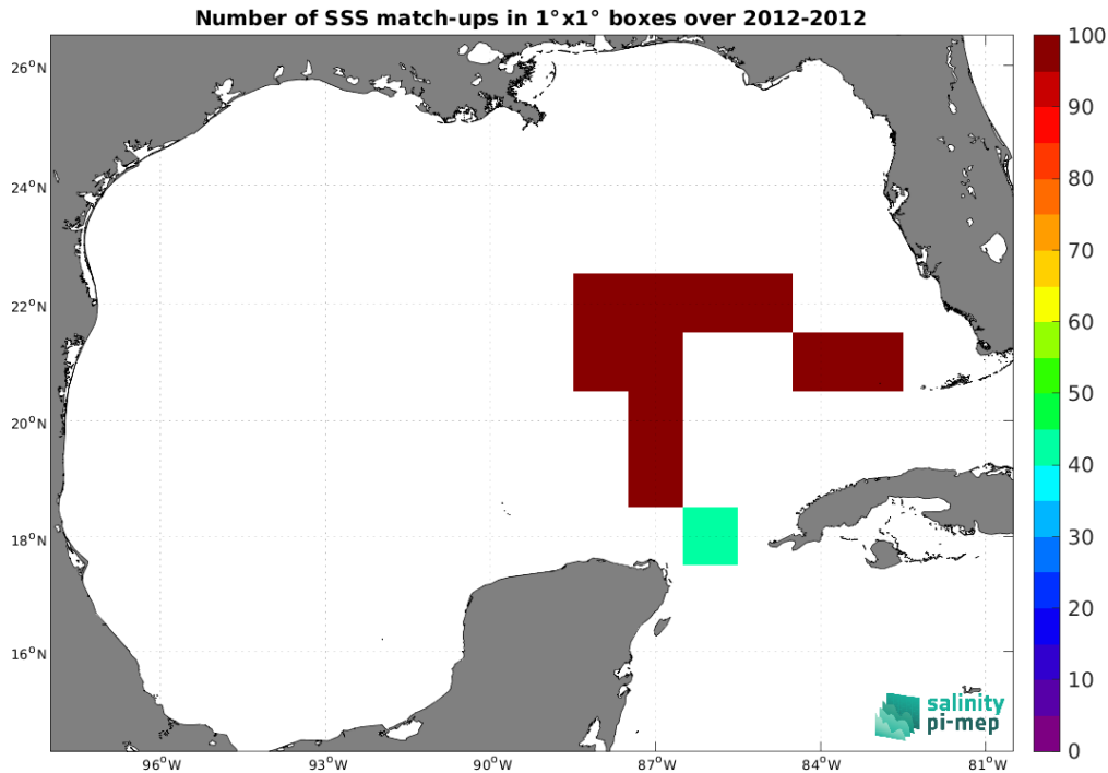
Figure 4: Number of SSS match-ups between TSG (GOSUD-Sailing-ship) SSS and the Aquarius SSS L3 OR v5 - Monthly - Rain mask (NASA-GSFC) SSS product for the Gulf of Mexico Pi-MEP region over 1^\circ \times 1^\circ boxes and for the full satellite product period.
