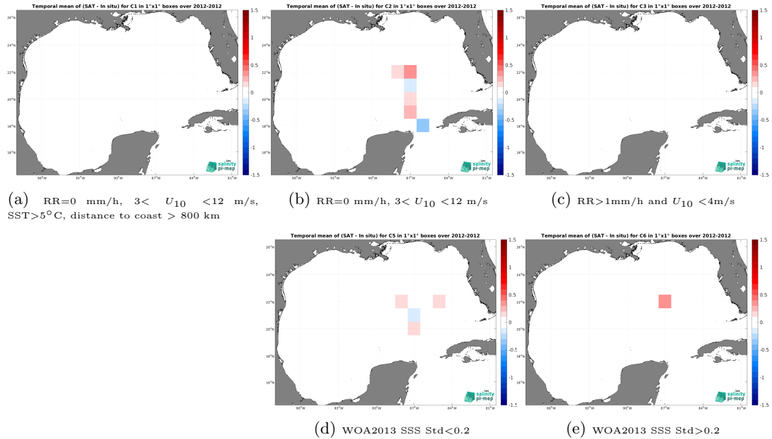
Figure 12: Temporal mean gridded over spatial boxes of size 1^\circ \times 1^\circ of \Delta SSS (Aquarius SSS L3 OR v5 - Monthly - Rain mask (NASA-GSFC) - TSG (GOSUD-Sailing-ship)) for 5 different subdatasets corresponding to:RR=0 mm/h, 3 < U_{10} < 12 m/s, SST >5^\circ\text{C} , distance to coast > 800 km (a), RR=0 mm/h, 3 < U_{10} < 12 m/s (b), RR >1 mm/h and U_{10} < 4 m/s (c), WOA2013 SSS Std <0.2 (d), WOA2013 SSS Std >0.2 (e).
