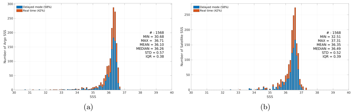
Figure 3: Histograms of SSS from Argo (a) and Aquarius SSS L3 OR v5 - Monthly - Rain mask (NASA-GSFC) (b) considering all match-up pairs per bins of 0.1 over the Gulf of Mexico Pi-MEP region and for the full satellite product period.
