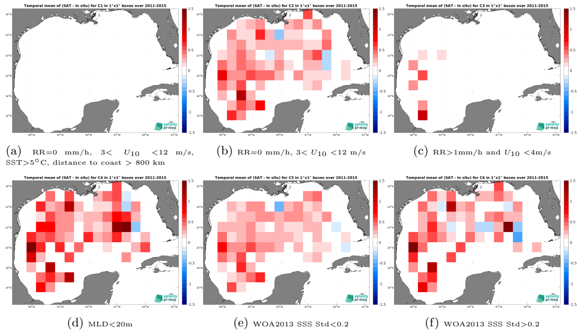
Figure 14: Temporal mean gridded over spatial boxes of size 1^\circ \times 1^\circ of \Delta SSS (Aquarius SSS L3 OR v5 - Monthly - Rain mask (NASA-GSFC) - Argo) for 6 different subdatasets corresponding to:RR=0 mm/h, 3 < U_{10} < 12 m/s, SST > 5^\circ\text{C} , distance to coast > 800 km (a), RR=0 mm/h, 3 < U_{10} < 12 m/s (b), RR > 1 mm/h and U_{10} < 4 m/s (c),MLD < 20 m (d),WOA2013 SSS Std < 0.2 (e),WOA2013 SSS Std > 0.2 (f).
