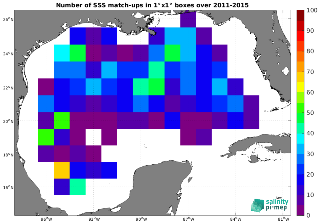
Figure 5: Number of SSS match-ups between Argo SSS and the Aquarius SSS L3 OR v5 - Monthly - Rain mask (NASA-GSFC) SSS product for the Gulf of Mexico Pi-MEP region over 1^\circ \times 1^\circ boxes and for the full satellite product period.
