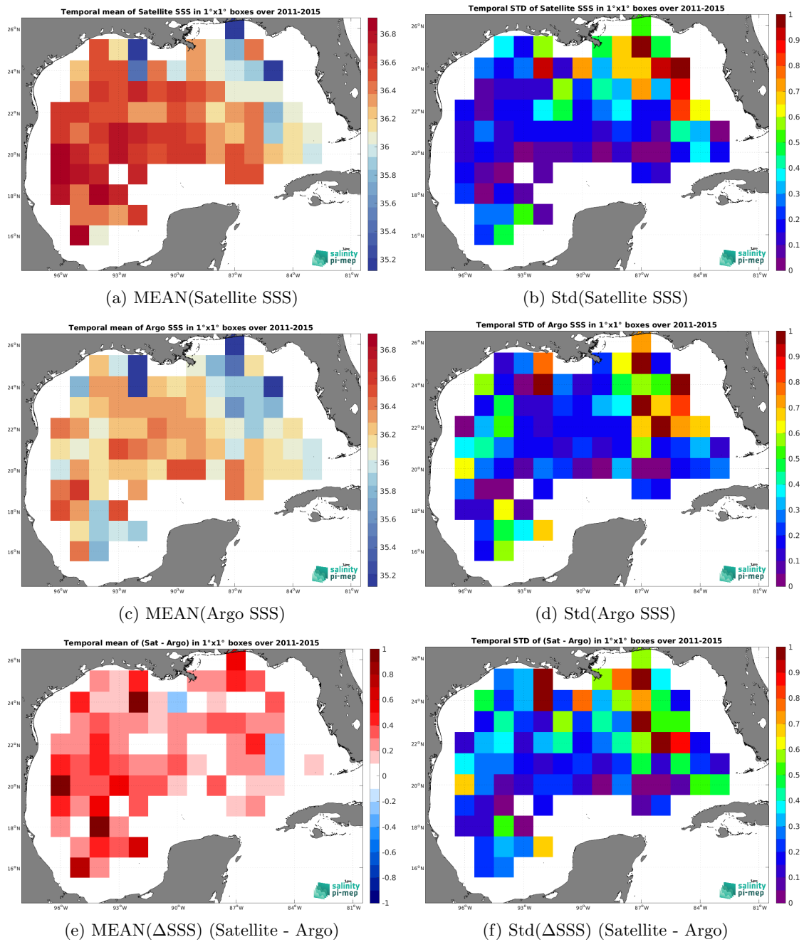
Figure 7: Temporal mean (left) and Std (right) of SSS from Aquarius SSS L3 OR v5 - Monthly - Rain mask (NASA-GSFC) (top), Argo (middle), and of \Delta SSS (Satellite - Argo). Only match-up pairs are used to generate these maps.
