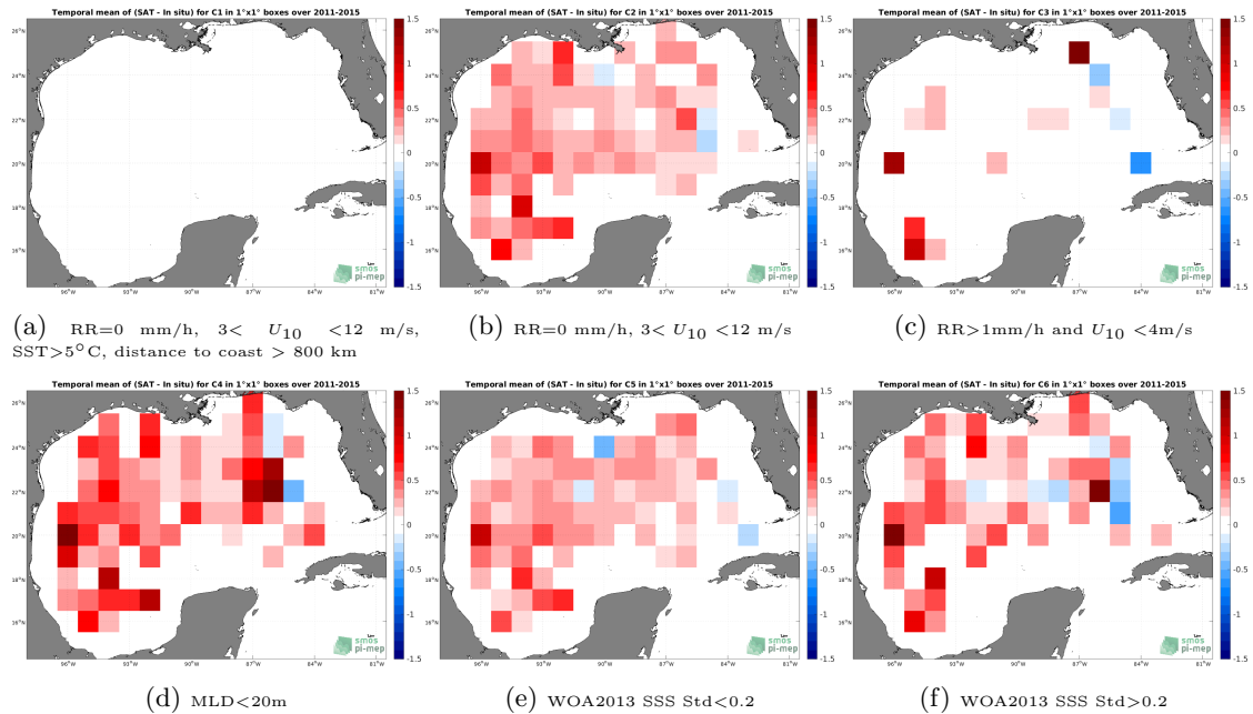
Figure 12: Temporal mean gridded over spatial boxes of size 1^\circ \times 1^\circ of \Delta SSS (Aquarius SSS L3 OR v5 - Monthly - Rain mask (NASA-GSFC) - Argo) for 6 different subdatasets corresponding to:RR=0 mm/h, 3 < U_{10} < 12 m/s, SST > 5^\circ\text{C} , distance to coast > 800 km (a), RR=0 mm/h, 3 < U_{10} < 12 m/s (b), RR > 1 mm/h and U_{10} < 4 m/s (c),MLD < 20 m (d),WOA2013 SSS Std < 0.2 (e),WOA2013 SSS Std > 0.2 (f).
