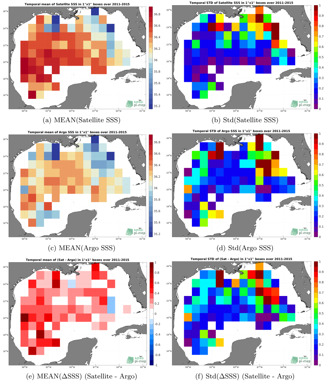
Figure 6: Temporal mean (left) and Std (right) of SSS from Aquarius SSS L3 OR v5 - Monthly - Rain mask (NASA-GSFC) (top), Argo (middle), and of \Delta SSS (Satellite - Argo). Only match-up pairs are used to generate these maps.
