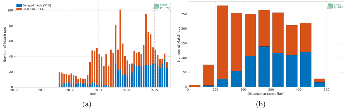
Figure 1: Number of match-ups between Argo and Aquarius SSS L3 OR v5 - Monthly - Rain mask (NASA-GSFC) SSS as a function of time (a) and as function of the distance to coast (b) over the Gulf of Mexico Pi-MEP region and for the full satellite product period.
