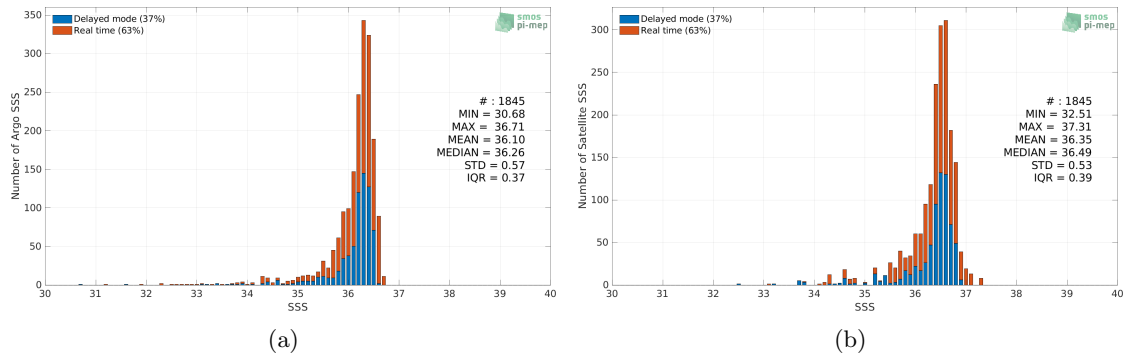
Figure 2: Histograms of SSS from Argo (a) and Aquarius SSS L3 OR v5 - Monthly - Rain mask (NASA-GSFC) (b) considering all match-up pairs per bins of 0.1 over the Gulf of Mexico Pi-MEP region and for the full satellite product period.
