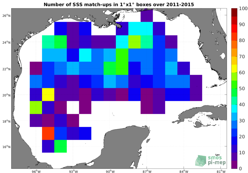
Figure 4: Number of SSS match-ups between Argo SSS and the Aquarius SSS L3 OR v5 - Monthly - Rain mask (NASA-GSFC) SSS product for the Gulf of Mexico Pi-MEP region over 1^\circ \times 1^\circ boxes and for the full satellite product period.
