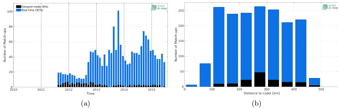
Figure 1: Number of match-ups between Argo and Aquarius-L3-OR-V5-MONTHLY-RAIN-MASK-1DEG SSS as a function of time (a) and as function of the distance to coast (b) over the Gulf of Mexico Pi-MEP region and for the full satellite product period.
