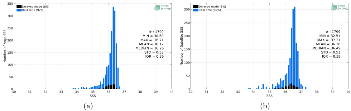
Figure 2: Histograms of SSS from Argo (a) and Aquarius-L3-OR-V5-MONTHLY-RAIN-MASK-1DEG (b) considering all match-up pairs per bins of 0.1 over the Gulf of Mexico Pi-MEP region and for the full satellite product period.
