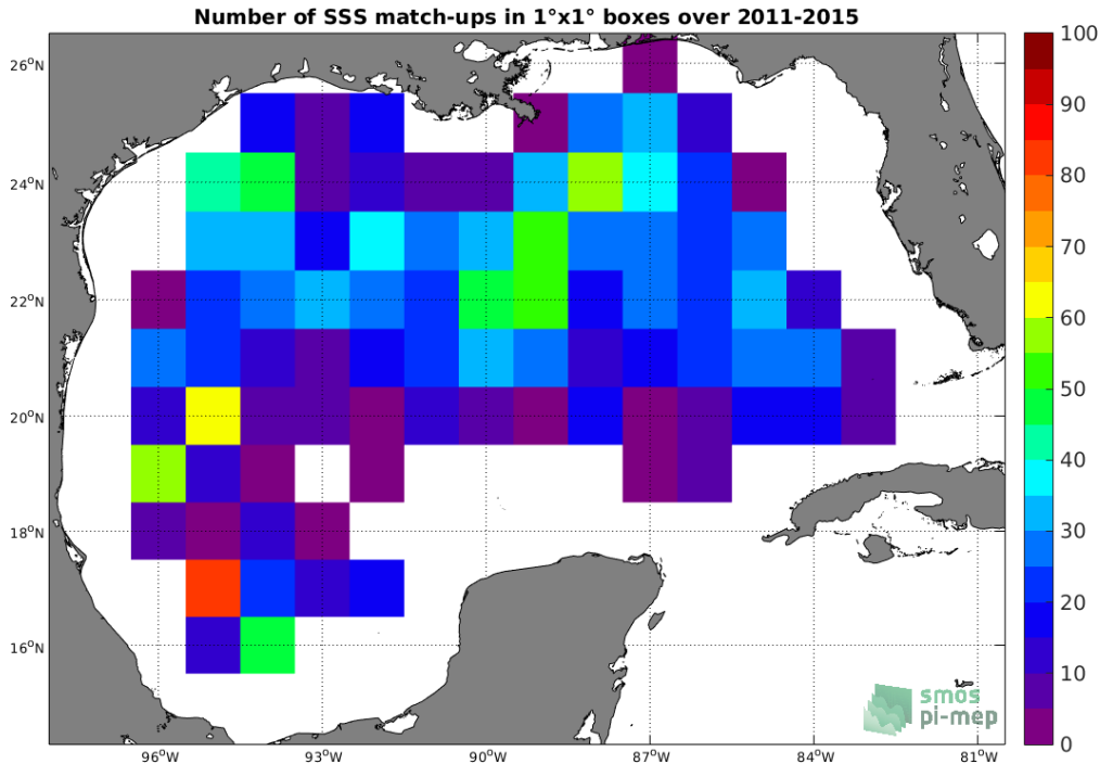
Figure 4: Number of SSS match-ups between Argo SSS and the Aquarius-L3-OR-V5-MONTHLY-RAIN-MASK-1DEG SSS product for the Gulf of Mexico Pi-MEP region over 1°x1° boxes and for the full satellite product period.
