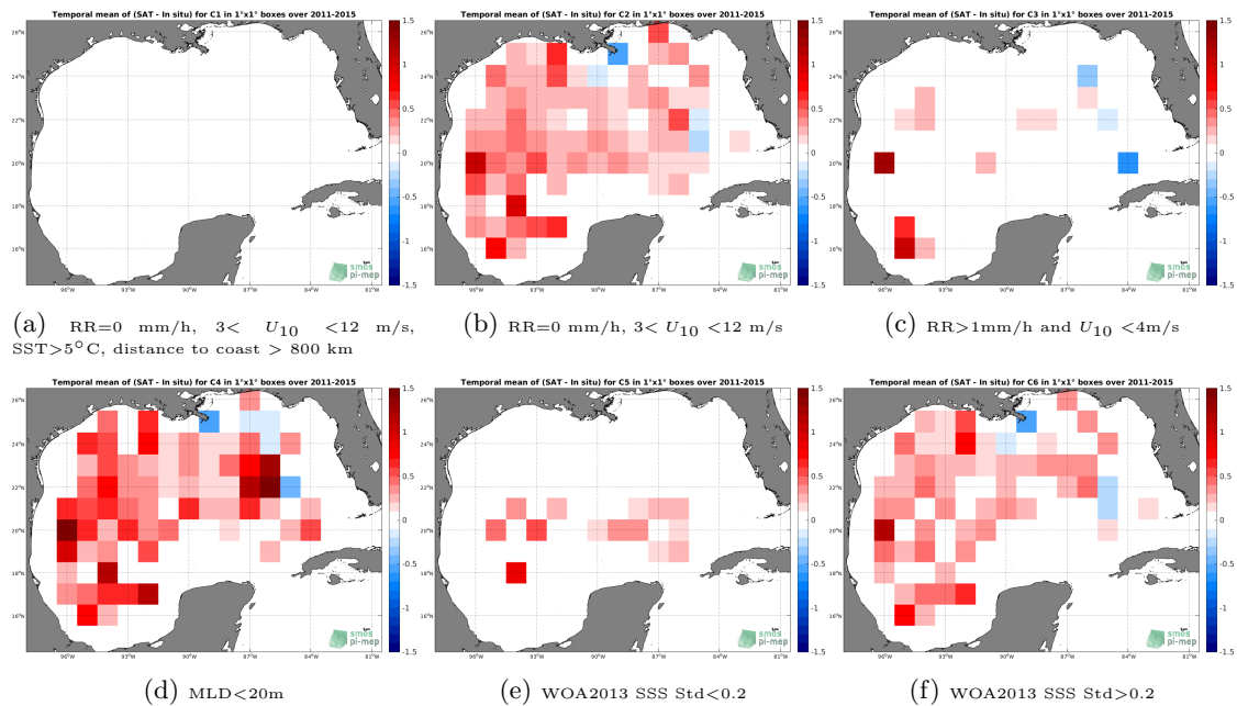
Figure 12: Temporal mean gridded over spatial boxes of size 1^\circ \times 1^\circ of \Delta SSS (Aquarius-L3-OR-V5-MONTHLY-RAIN-MASK-1DEG - Argo) for 6 different subdatasets corresponding to:RR=0 mm/h, 3 < U_{10} < 12 m/s, SST >5^\circ C, distance to coast > 800 km (a), RR=0 mm/h, 3 < U_{10} < 12 m/s (b), RR >1 mm/h and U_{10} < 4 m/s (c),MLD <20 m (d),WOA2013 SSS Std <0.2 (e),WOA2013 SSS Std >0.2 (f).
