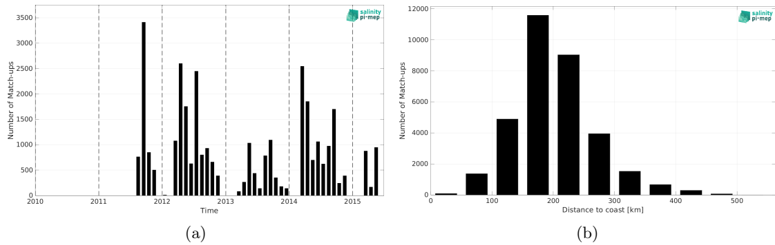
Figure 2: Number of match-ups between TSG (SAMOS) and Aquarius SSS L3 CAP v5 - 7-Day running (JPL) SSS as a function of time (a) and as function of the distance to coast (b) over the Gulf of Mexico Pi-MEP region and for the full satellite product period.
