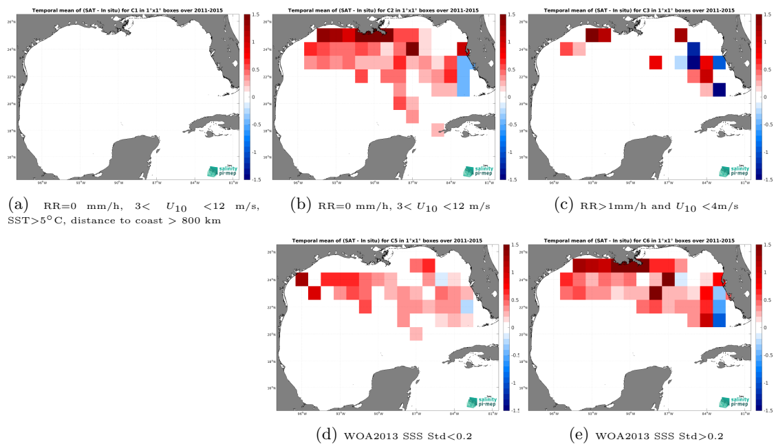
Figure 14: Temporal mean gridded over spatial boxes of size 1^\circ \times 1^\circ of \Delta\text{SSS} (Aquarius SSS L3 CAP v5 - 7-Day running (JPL) - TSG (SAMOS)) for 5 different subdatasets corresponding to:RR=0 mm/h, 3 < U_{10} < 12 m/s, SST >5^\circ\text{C} , distance to coast > 800 km (a), RR=0 mm/h, 3 < U_{10} < 12 m/s (b), RR >1 mm/h and U_{10} < 4 m/s (c), WOA2013 SSS Std <0.2 (d), WOA2013 SSS Std >0.2 (e).
