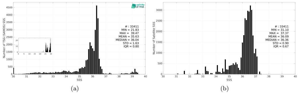
Figure 3: Histograms of SSS from TSG (SAMOS) (a) and Aquarius SSS L3 CAP v5 - 7-Day running (JPL) (b) considering all match-up pairs per bins of 0.1 over the Gulf of Mexico Pi-MEP region and for the full satellite product period.
