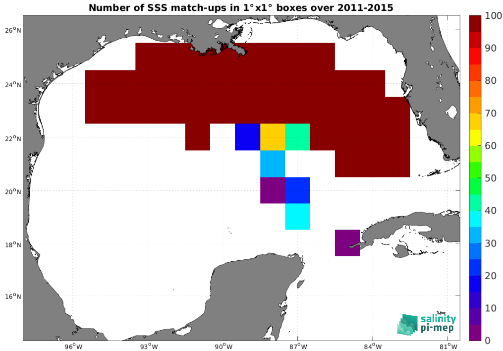
Figure 5: Number of SSS match-ups between TSG (SAMOS) SSS and the Aquarius SSS L3 CAP v5 - 7-Day running (JPL) SSS product for the Gulf of Mexico Pi-MEP region over 1°×1° boxes and for the full satellite product period.
