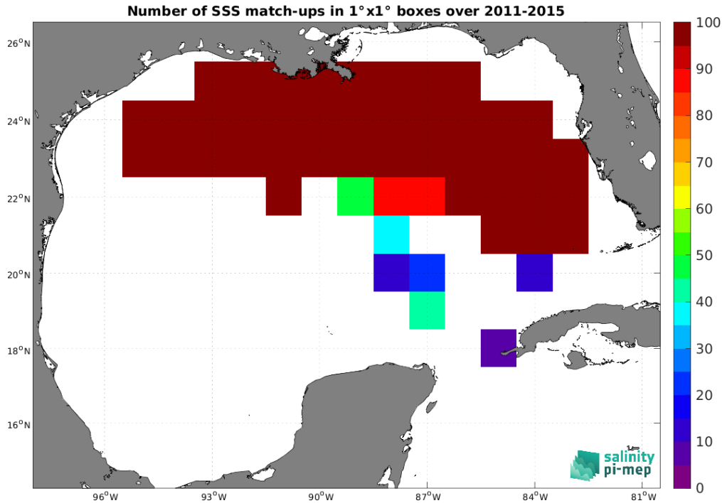
Figure 4: Number of SSS match-ups between TSG (SAMOS) SSS and the Aquarius SSS L3 CAP v5 - 7-Day running (JPL) SSS product for the Gulf of Mexico Pi-MEP region over 1°×1° boxes and for the full satellite product period.
