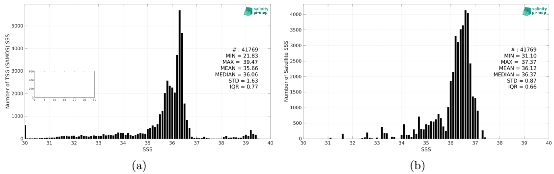
Figure 2: Histograms of SSS from TSG (SAMOS) (a) and Aquarius SSS L3 CAP v5 - 7-Day running (JPL) (b) considering all match-up pairs per bins of 0.1 over the Gulf of Mexico Pi-MEP region and for the full satellite product period.
