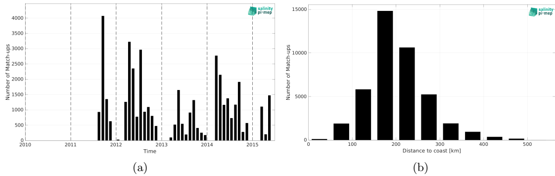
Figure 1: Number of match-ups between TSG (SAMOS) and Aquarius SSS L3 CAP v5 - 7-Day running (JPL) SSS as a function of time (a) and as function of the distance to coast (b) over the Gulf of Mexico Pi-MEP region and for the full satellite product period.
