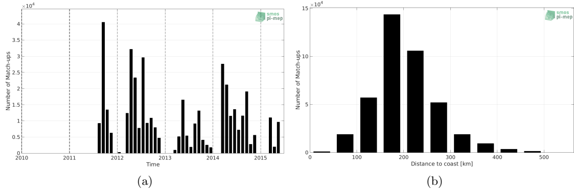
Figure 1: Number of match-ups between TSG (SAMOS) and Aquarius SSS L3 CAP v5 - 7-Day running (JPL) SSS as a function of time (a) and as function of the distance to coast (b) over the Gulf of Mexico Pi-MEP region and for the full satellite product period.
