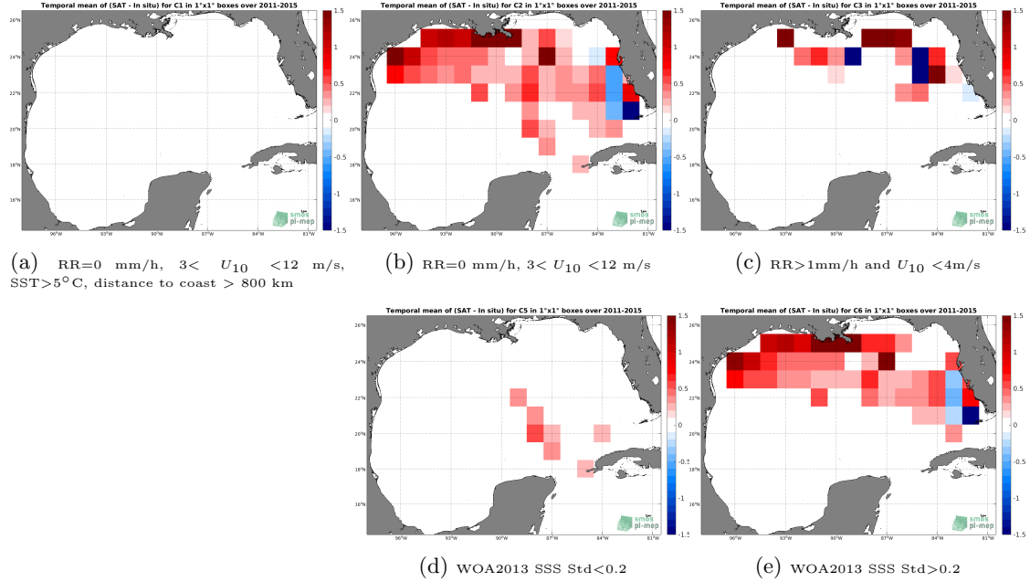
Figure 12: Temporal mean gridded over spatial boxes of size 1^{\circ}\times 1^{\circ} of \Delta\text{SSS} (Aquarius SSS L3 CAP v5 - 7-Day running (JPL) - TSG (SAMOS)) for 5 different subdatasets corresponding to: RR=0 mm/h, 3 < U_{10} < 12 m/s, SST >5^{\circ}\text{C} , distance to coast > 800 km (a), RR=0 mm/h, 3 < U_{10} < 12 m/s (b), RR >1 mm/h and U_{10} < 4 m/s (c), WOA2013 SSS Std <0.2 (d), WOA2013 SSS Std >0.2 (e).
