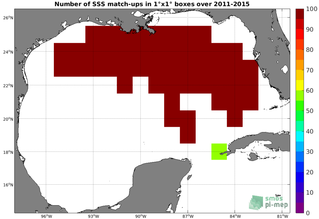
Figure 4: Number of SSS match-ups between TSG (SAMOS) SSS and the Aquarius SSS L3 CAP v5 - 7-Day running (JPL) SSS product for the Gulf of Mexico Pi-MEP region over 1^\circ \times 1^\circ boxes and for the full satellite product period.
