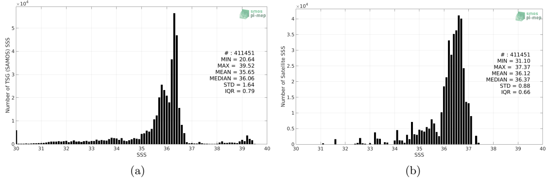
Figure 2: Histograms of SSS from TSG (SAMOS) (a) and Aquarius SSS L3 CAP v5 - 7-Day running (JPL) (b) considering all match-up pairs per bins of 0.1 over the Gulf of Mexico Pi-MEP region and for the full satellite product period.
