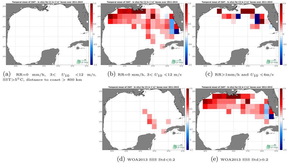
Figure 12: Temporal mean gridded over spatial boxes of size 1^{\circ}\times 1^{\circ} of \Delta\text{SSS} (Aquarius-L3-JPL-V5-7DAY-RUNNING - TSG-SAMOS) for 5 different subdatasets corresponding to: RR=0 mm/h, 3 < U_{10} < 12 m/s, SST > 5^{\circ}\text{C} , distance to coast > 800 km (a), RR=0 mm/h, 3 < U_{10} < 12 m/s (b), RR > 1 mm/h and U_{10} < 4 m/s (c), WOA2013 SSS Std < 0.2 (d), WOA2013 SSS Std > 0.2 (e).
