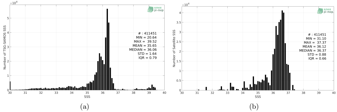
Figure 2: Histograms of SSS from TSG-SAMOS (a) and Aquarius-L3-JPL-V5-7DAY-RUNNING (b) considering all match-up pairs per bins of 0.1 over the Gulf of Mexico Pi-MEP region and for the full satellite product period.
