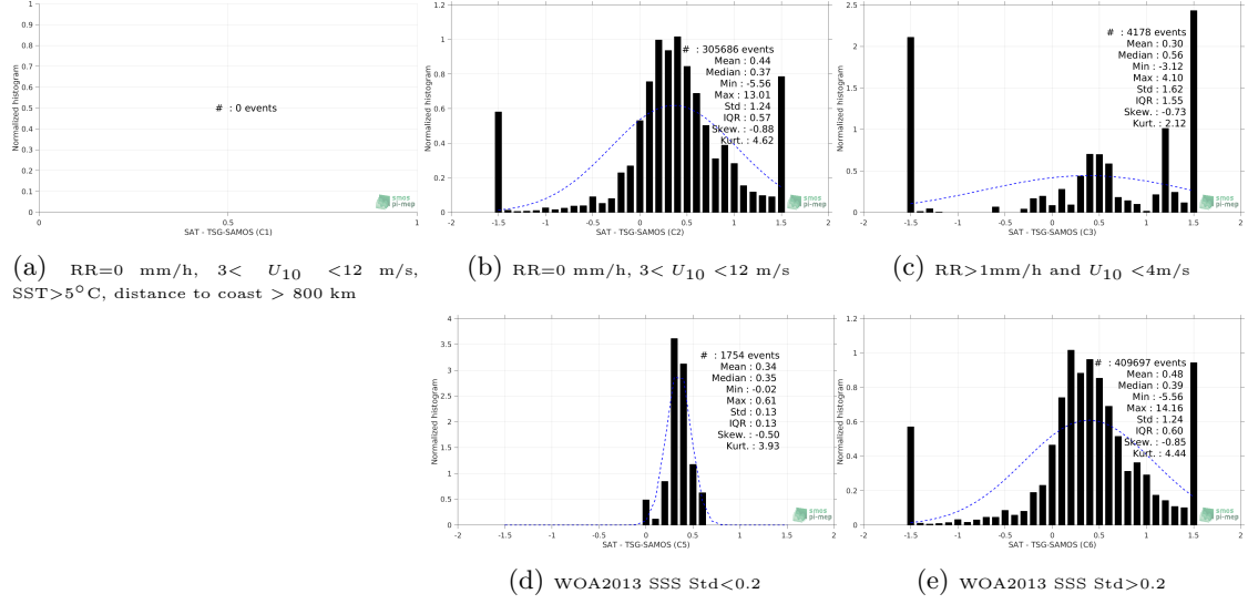
Figure 13: Normalized histogram of \Delta\text{SSS} (Aquarius-L3-JPL-V5-7DAY-RUNNING - TSG-SAMOS) for 5 different subdatasets corresponding to: RR=0 mm/h, 3 < U_{10} < 12 m/s, SST > 5^{\circ}\text{C} , distance to coast > 800 km (a), RR=0 mm/h, 3 < U_{10} < 12 m/s (b), RR > 1\text{mm/h} and U_{10} < 4\text{m/s} (c), WOA2013 SSS Std < 0.2 (d), WOA2013 SSS Std > 0.2 (e).
