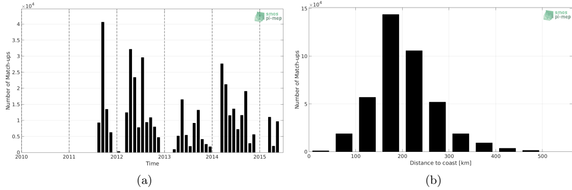
Figure 1: Number of match-ups between TSG-SAMOS and Aquarius-L3-JPL-V5-7DAY-RUNNING SSS as a function of time (a) and as function of the distance to coast (b) over the Gulf of Mexico Pi-MEP region and for the full satellite product period.
