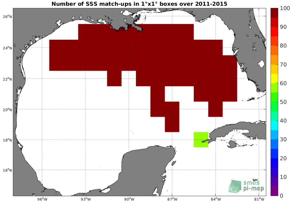
Figure 4: Number of SSS match-ups between TSG-SAMOS SSS and the Aquarius-L3-JPL-V5-7DAY-RUNNING SSS product for the Gulf of Mexico Pi-MEP region over 1^\circ \times 1^\circ boxes and for the full satellite product period.
