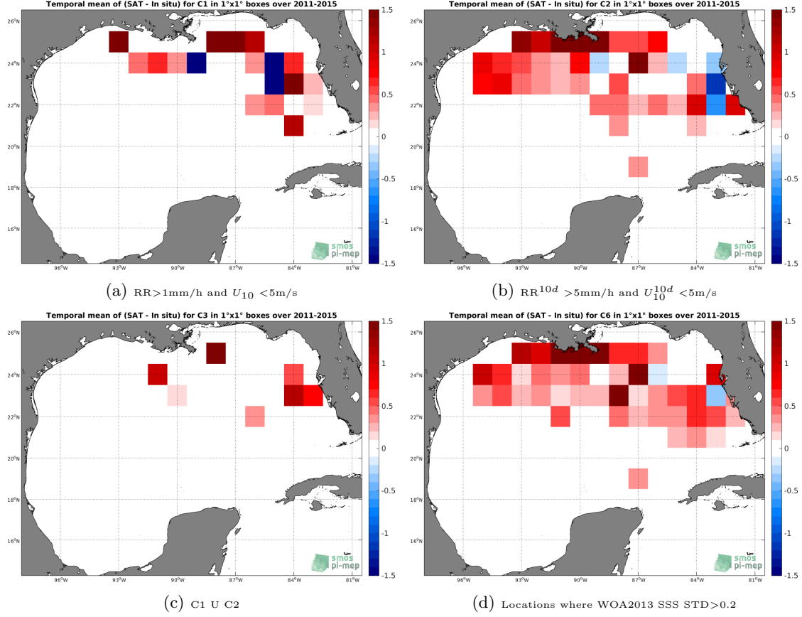
Figure 12: Temporal mean gridded over spatial boxes of size 1^\circ \times 1^\circ of \Delta SSS (Aquarius-L3-JPL-V5-7DAY-RUNNING - TSG-SAMOS) for 4 different subdatasets corresponding to: RR > 1\text{mm/h} and U_{10} < 5\text{m/s} (a), RR^{10d} > 5\text{mm/h} and U_{10}^{10d} < 5\text{m/s} (b), C1 U C2 (c), Locations where WOA2013 SSS STD > 0.2 (d).
