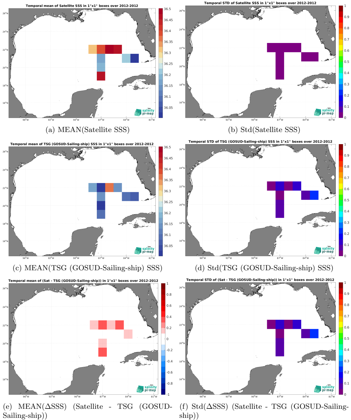
Figure 7: Temporal mean (left) and Std (right) of SSS from Aquarius SSS L3 CAP v5 - 7-Day running (JPL) (top), TSG (GOSUD-Sailing-ship) (middle), and of \Delta SSS (Satellite - TSG (GOSUD-Sailing-ship)). Only match-up pairs are used to generate these maps.
