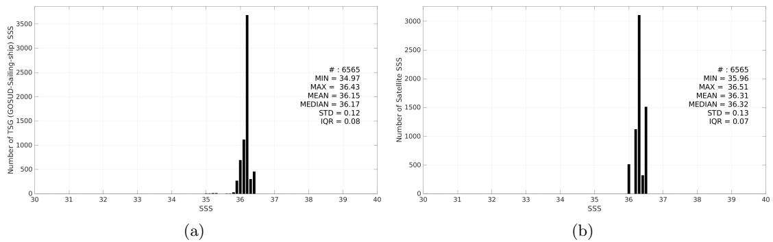
Figure 3: Histograms of SSS from TSG (GOSUD-Sailing-ship) (a) and Aquarius SSS L3 CAP v5 - 7-Day running (JPL) (b) considering all match-up pairs per bins of 0.1 over the Gulf of Mexico Pi-MEP region and for the full satellite product period.
