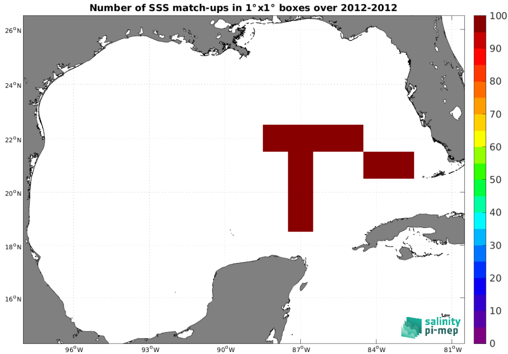
Figure 5: Number of SSS match-ups between TSG (GOSUD-Sailing-ship) SSS and the Aquarius SSS L3 CAP v5 - 7-Day running (JPL) SSS product for the Gulf of Mexico Pi-MEP region over 1^\circ \times 1^\circ boxes and for the full satellite product period.
