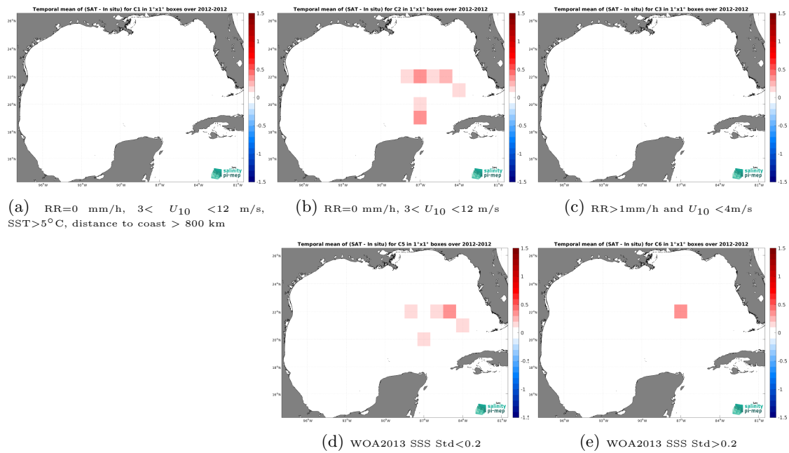
Figure 14: Temporal mean gridded over spatial boxes of size 1^\circ \times 1^\circ of \Delta\text{SSS} (Aquarius SSS L3 CAP v5 - 7-Day running (JPL) - TSG (GOSUD-Sailing-ship)) for 5 different subdatasets corresponding to:RR=0 mm/h, 3 < U_{10} < 12 m/s, SST >5^\circ\text{C} , distance to coast > 800 km (a), RR=0 mm/h, 3 < U_{10} < 12 m/s (b), RR >1 mm/h and U_{10} < 4 m/s (c), WOA2013 SSS Std <0.2 (d), WOA2013 SSS Std >0.2 (e).
