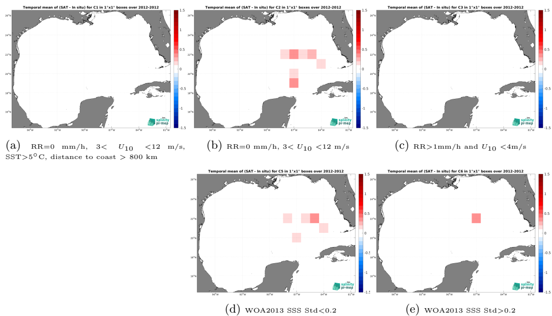
Figure 14: Temporal mean gridded over spatial boxes of size 1^\circ \times 1^\circ of \Delta SSS (Aquarius SSS L3 CAP v5 - 7-Day running (JPL) - TSG (GOSUD-Sailing-ship)) for 5 different subdatasets corresponding to:RR=0 mm/h, 3 < U_{10} < 12 m/s, SST >5^\circ C, distance to coast > 800 km (a), RR=0 mm/h, 3 < U_{10} < 12 m/s (b), RR >1 mm/h and U_{10} < 4 m/s (c), WOA2013 SSS Std <0.2 (d), WOA2013 SSS Std >0.2 (e).
