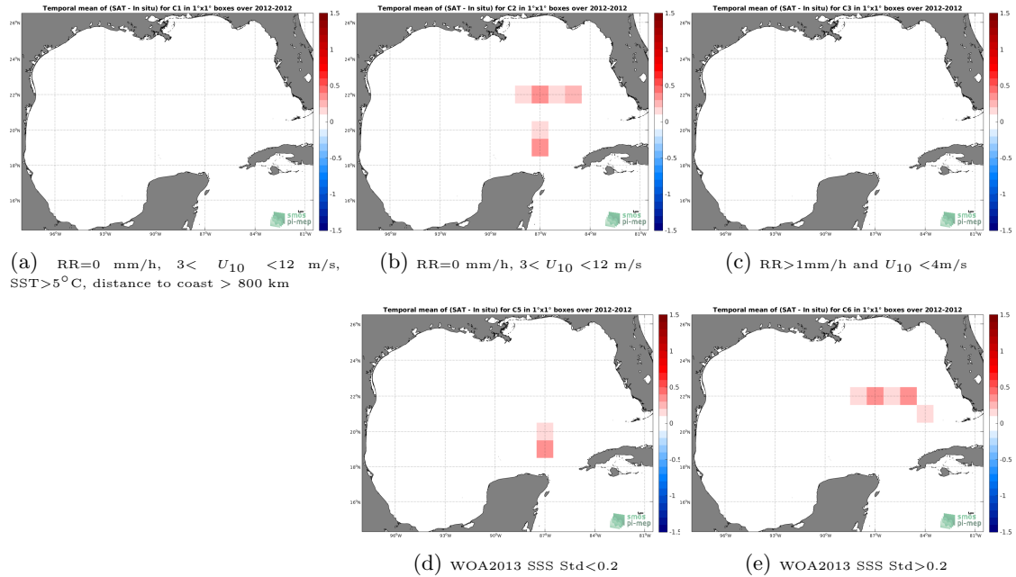
Figure 12: Temporal mean gridded over spatial boxes of size 1^\circ \times 1^\circ of \Delta SSS (Aquarius SSS L3 CAP v5 - 7-Day running (JPL) - TSG (GOSUD-Sailing-ship)) for 5 different subdatasets corresponding to:RR=0 mm/h, 3 < U_{10} < 12 m/s, SST >5^\circ\text{C} , distance to coast > 800 km (a), RR=0 mm/h, 3 < U_{10} < 12 m/s (b), RR >1 mm/h and U_{10} < 4 m/s (c), WOA2013 SSS Std <0.2 (d), WOA2013 SSS Std >0.2 (e).
