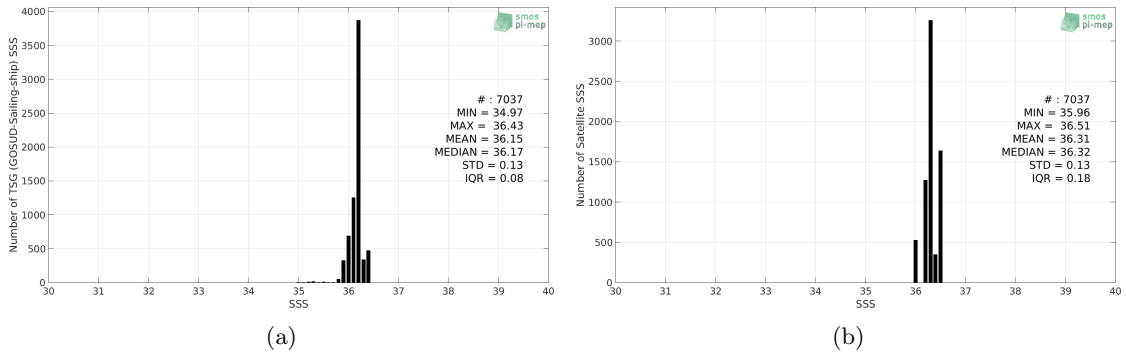
Figure 2: Histograms of SSS from TSG (GOSUD-Sailing-ship) (a) and Aquarius SSS L3 CAP v5 - 7-Day running (JPL) (b) considering all match-up pairs per bins of 0.1 over the Gulf of Mexico Pi-MEP region and for the full satellite product period.
