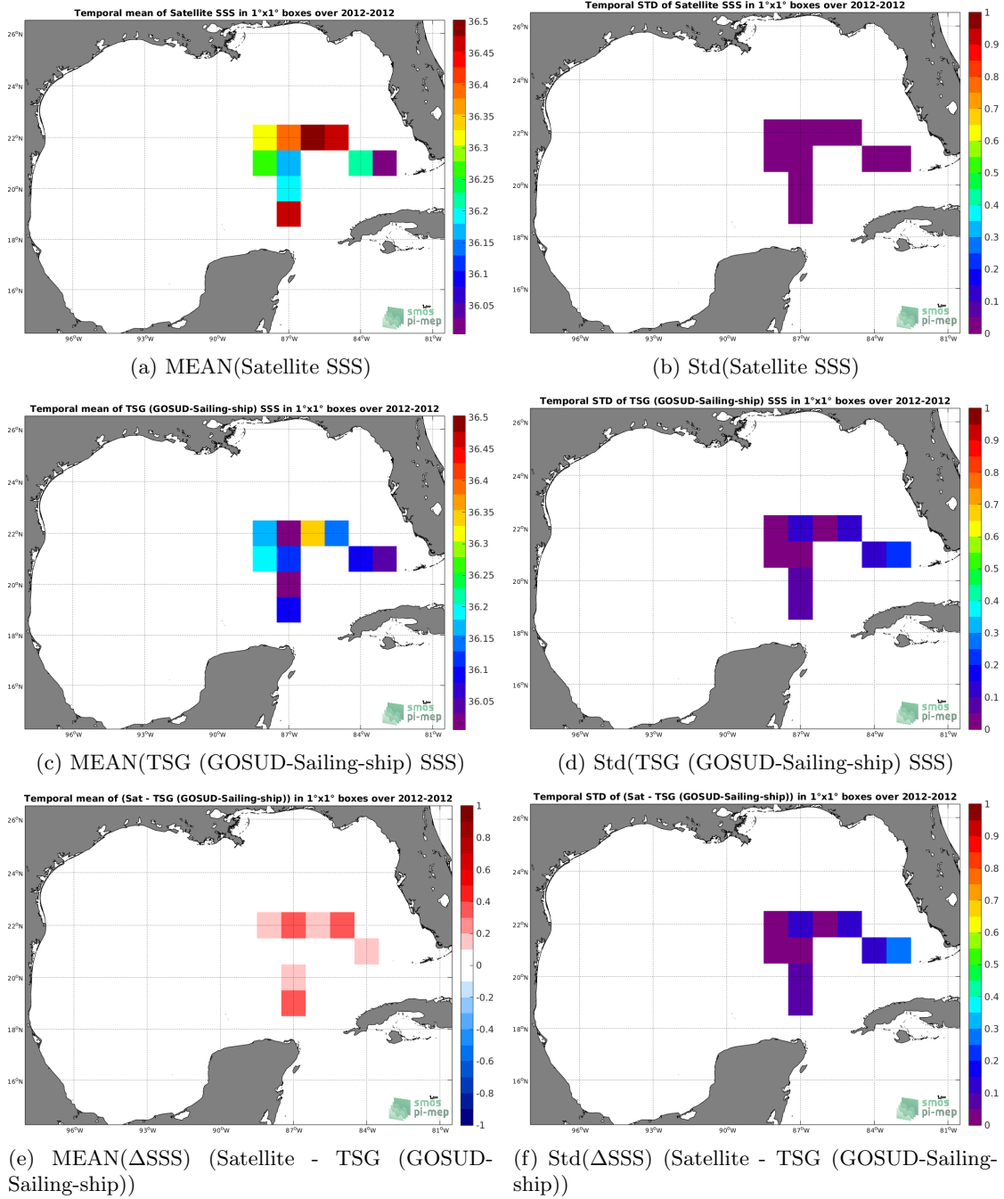
Figure 6: Temporal mean (left) and Std (right) of SSS from Aquarius SSS L3 CAP v5 - 7-Day running (JPL) (top), TSG (GOSUD-Sailing-ship) (middle), and of \Delta SSS (Satellite - TSG (GOSUD-Sailing-ship)). Only match-up pairs are used to generate these maps.
