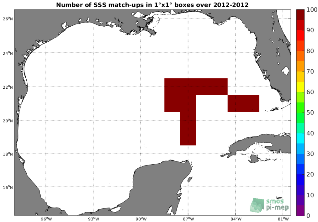
Figure 4: Number of SSS match-ups between TSG (GOSUD-Sailing-ship) SSS and the Aquarius SSS L3 CAP v5 - 7-Day running (JPL) SSS product for the Gulf of Mexico Pi-MEP region over 1^\circ \times 1^\circ boxes and for the full satellite product period.
