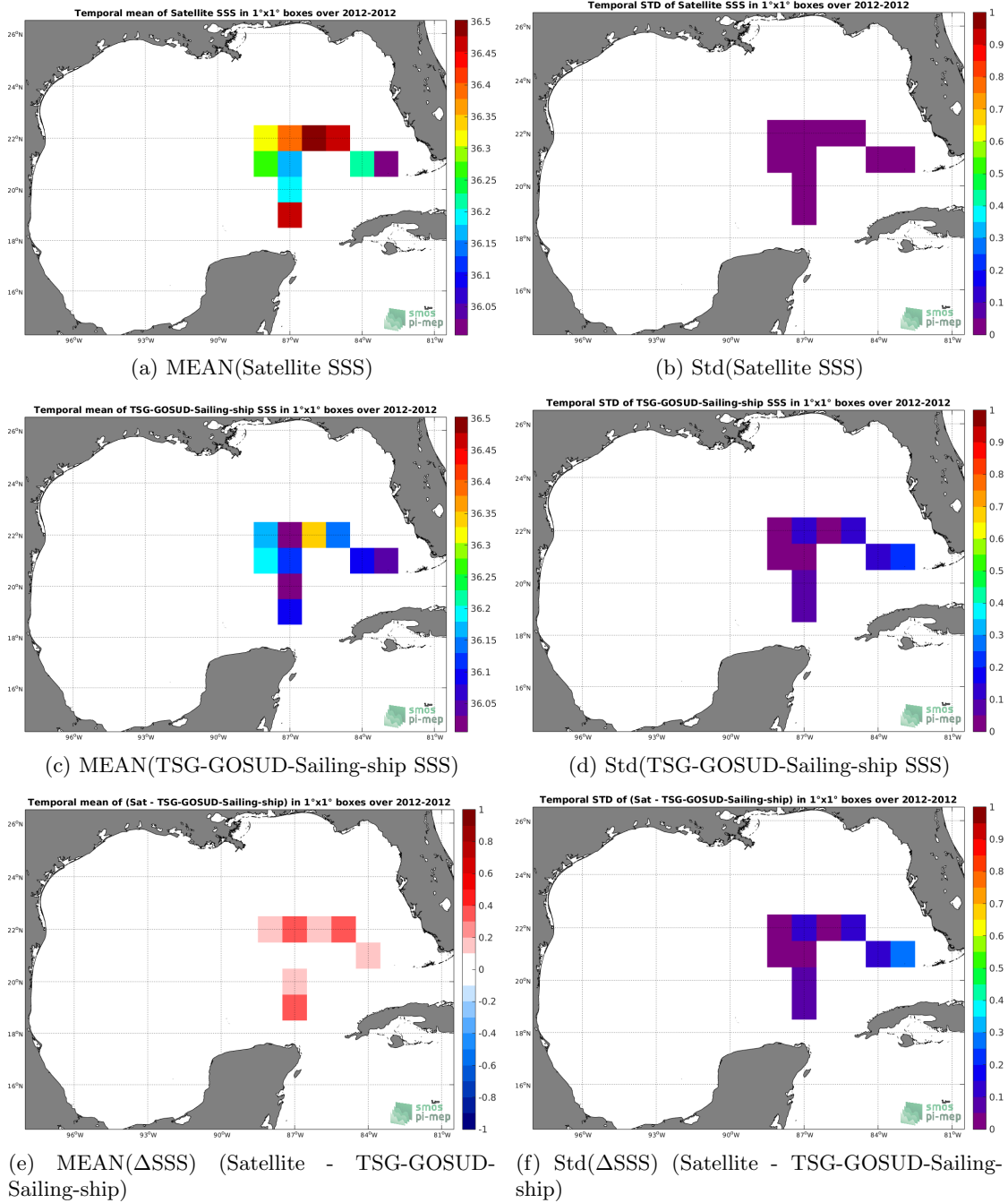
Figure 6: Temporal mean (left) and Std (right) of SSS from Aquarius-L3-JPL-V5-7DAY-RUNNING (top), TSG-GOSUD-Sailing-ship (middle), and of \Delta SSS (Satellite - TSG-GOSUD-Sailing-ship). Only match-up pairs are used to generate these maps.
