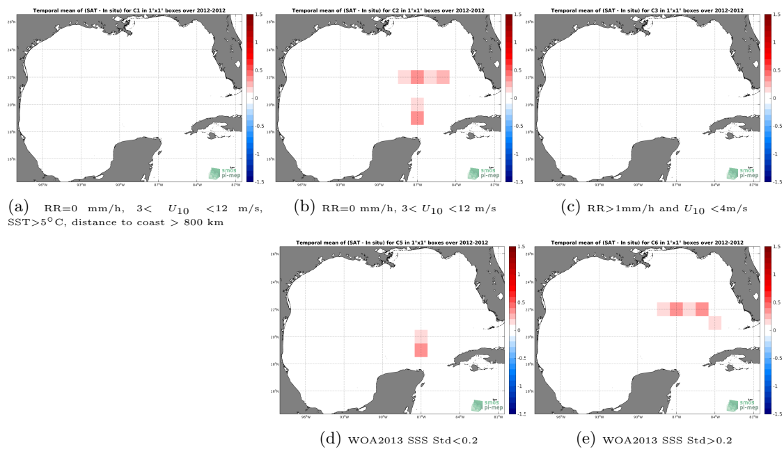
Figure 12: Temporal mean gridded over spatial boxes of size 1^\circ \times 1^\circ of \Delta SSS (Aquarius-L3-JPL-V5-7DAY-RUNNING - TSG-GOSUD-Sailing-ship) for 5 different subdatasets corresponding to:RR=0 mm/h, 3 < U_{10} < 12 m/s, SST >5^\circ C, distance to coast > 800 km (a), RR=0 mm/h, 3 < U_{10} < 12 m/s (b), RR >1 mm/h and U_{10} < 4 m/s (c), WOA2013 SSS Std <0.2 (d), WOA2013 SSS Std >0.2 (e).
