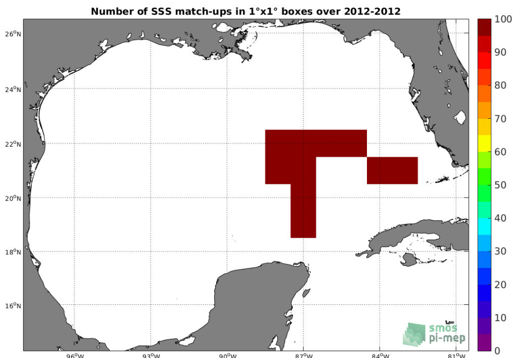
Figure 4: Number of SSS match-ups between TSG-GOSUD-Sailing-ship SSS and the Aquarius-L3-JPL-V5-7DAY-RUNNING SSS product for the Gulf of Mexico Pi-MEP region over 1°x1° boxes and for the full satellite product period.
