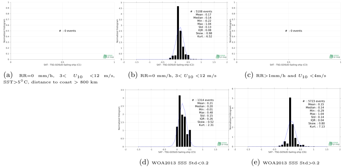
Figure 13: Normalized histogram of \Delta SSS (Aquarius-L3-JPL-V5-7DAY-RUNNING - TSG-GOSUD-Sailing-ship) for 5 different subdatasets corresponding to: RR=0 mm/h, 3 < U_{10} < 12 m/s, SST > 5°C, distance to coast > 800 km (a), RR=0 mm/h, 3 < U_{10} < 12 m/s (b), RR > 1mm/h and U_{10} < 4 m/s (c), WOA2013 SSS Std < 0.2 (d), WOA2013 SSS Std > 0.2 (e).
