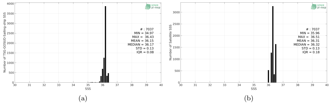
Figure 2: Histograms of SSS from TSG-GOSUD-Sailing-ship (a) and Aquarius-L3-JPL-V5-7DAY-RUNNING (b) considering all match-up pairs per bins of 0.1 over the Gulf of Mexico Pi-MEP region and for the full satellite product period.
