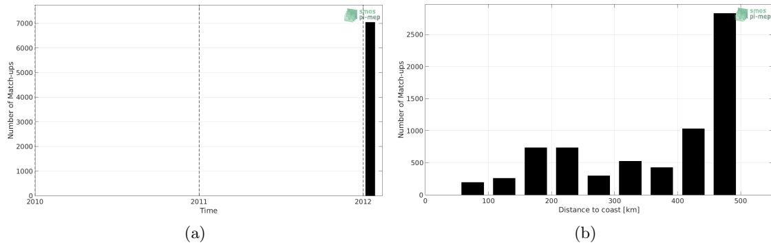
Figure 1: Number of match-ups between TSG-GOSUD-Sailing-ship and Aquarius-L3-JPL-V5-7DAY-RUNNING SSS as a function of time (a) and as function of the distance to coast (b) over the Gulf of Mexico Pi-MEP region and for the full satellite product period.
