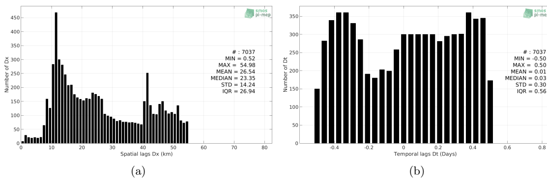
Figure 5: Histograms of the spatial (a) and temporal (b) lags between the time of the TSG-GOSUD-Sailing-ship measurements and the date of the corresponding Aquarius-L3-JPL-V5-7DAY-RUNNING SSS product.
