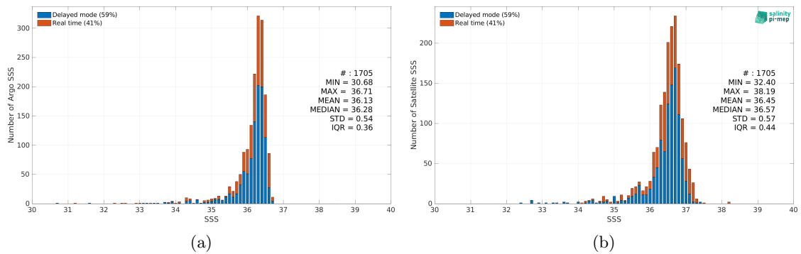
Figure 2: Histograms of SSS from Argo (a) and Aquarius SSS L3 CAP v5 - 7-Day running (JPL) (b) considering all match-up pairs per bins of 0.1 over the Gulf of Mexico Pi-MEP region and for the full satellite product period.
