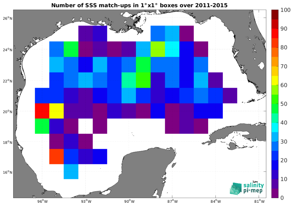
Figure 4: Number of SSS match-ups between Argo SSS and the Aquarius SSS L3 CAP v5 - 7-Day running (JPL) SSS product for the Gulf of Mexico Pi-MEP region over 1^\circ \times 1^\circ boxes and for the full satellite product period.
