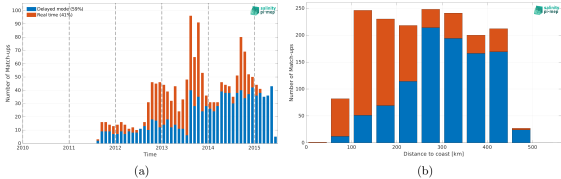
Figure 1: Number of match-ups between Argo and Aquarius SSS L3 CAP v5 - 7-Day running (JPL) SSS as a function of time (a) and as function of the distance to coast (b) over the Gulf of Mexico Pi-MEP region and for the full satellite product period.
