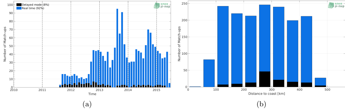
Figure 1: Number of match-ups between Argo and Aquarius-L3-JPL-V5-7DAY-RUNNING SSS as a function of time (a) and as function of the distance to coast (b) over the Gulf of Mexico Pi-MEP region and for the full satellite product period.
