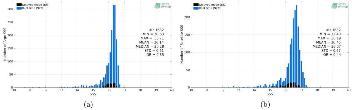
Figure 2: Histograms of SSS from Argo (a) and Aquarius-L3-JPL-V5-7DAY-RUNNING (b) considering all match-up pairs per bins of 0.1 over the Gulf of Mexico Pi-MEP region and for the full satellite product period.
