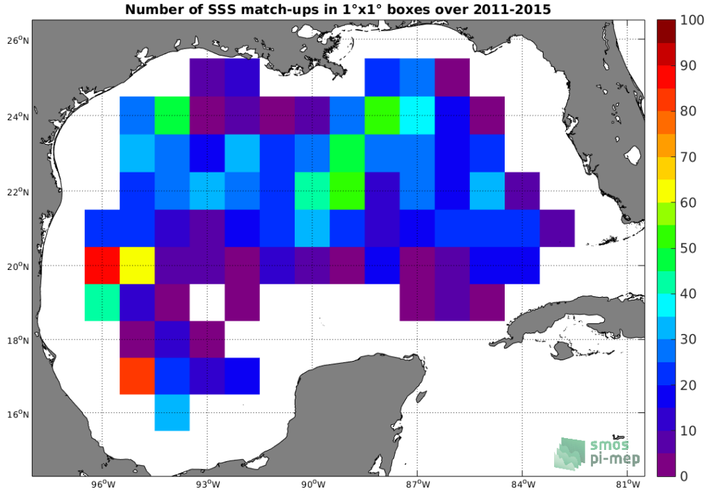
Figure 4: Number of SSS match-ups between Argo SSS and the Aquarius-L3-JPL-V5-7DAY-RUNNING SSS product for the Gulf of Mexico Pi-MEP region over 1^\circ \times 1^\circ boxes and for the full satellite product period.
