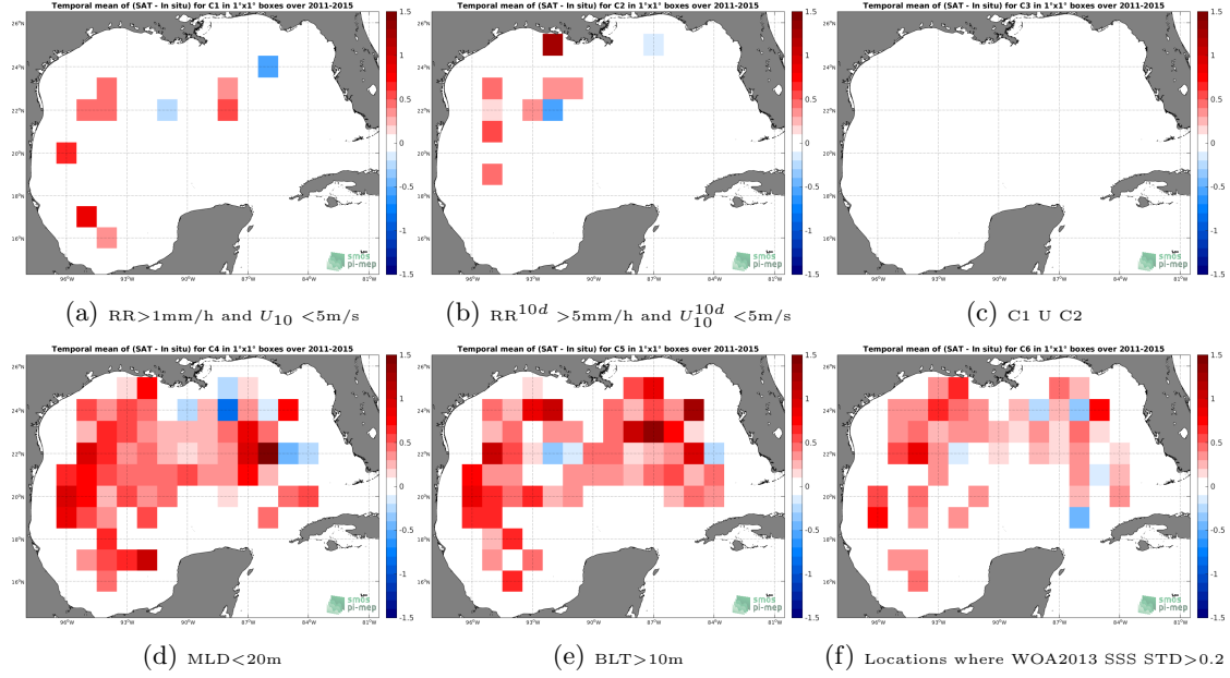
Figure 12: Temporal mean gridded over spatial boxes of size 1^\circ \times 1^\circ of \Delta\text{SSS} (Aquarius-L3-JPL-V5-7DAY-RUNNING - Argo) for 6 different subdatasets corresponding to: \text{RR} > 1\text{mm/h} and U_{10} < 5\text{m/s} (a), \text{RR}^{10d} > 5\text{mm/h} and U_{10}^{10d} < 5\text{m/s} (b), C1 U C2 (c), \text{MLD} < 20\text{m} (d), \text{BLT} > 10\text{m} (e), Locations where WOA2013 SSS STD > 0.2 (f).
