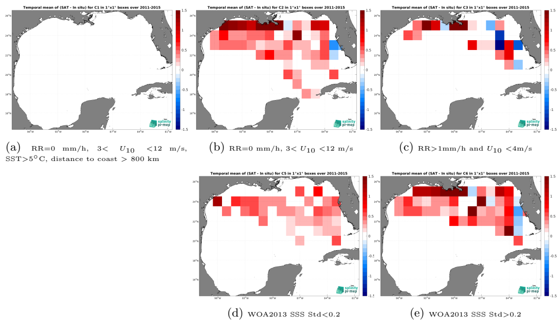
Figure 14: Temporal mean gridded over spatial boxes of size 1^\circ \times 1^\circ of \Delta SSS (Aquarius SSS L3 CAP v5 - Monthly (JPL) - TSG (SAMOS)) for 5 different subdatasets corresponding to:RR=0 mm/h, 3 < U_{10} < 12 m/s, SST > 5^\circ\text{C} , distance to coast > 800 km (a), RR=0 mm/h, 3 < U_{10} < 12 m/s (b), RR > 1 mm/h and U_{10} < 4 m/s (c), WOA2013 SSS Std < 0.2 (d), WOA2013 SSS Std > 0.2 (e).
