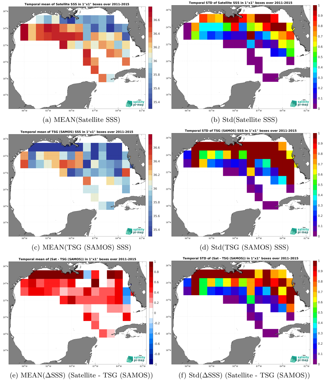
Figure 7: Temporal mean (left) and Std (right) of SSS from Aquarius SSS L3 CAP v5 - Monthly (JPL) (top), TSG (SAMOS) (middle), and of \Delta SSS (Satellite - TSG (SAMOS)). Only match-up pairs are used to generate these maps.
