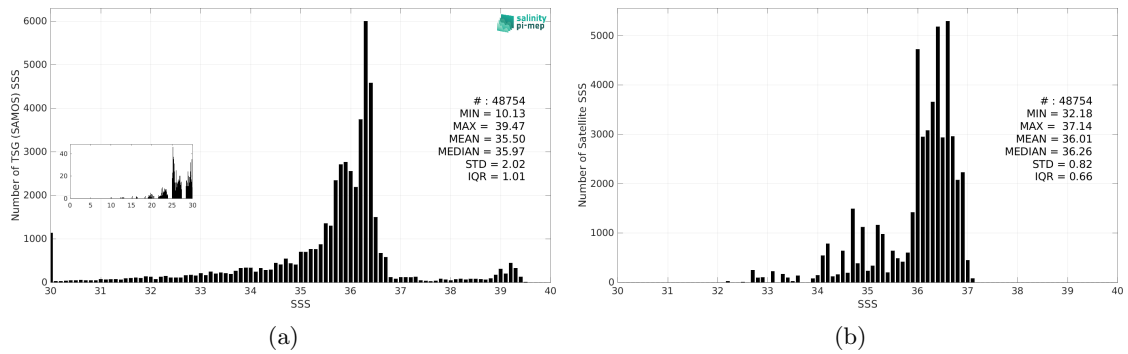
Figure 3: Histograms of SSS from TSG (SAMOS) (a) and Aquarius SSS L3 CAP v5 - Monthly (JPL) (b) considering all match-up pairs per bins of 0.1 over the Gulf of Mexico Pi-MEP region and for the full satellite product period.
