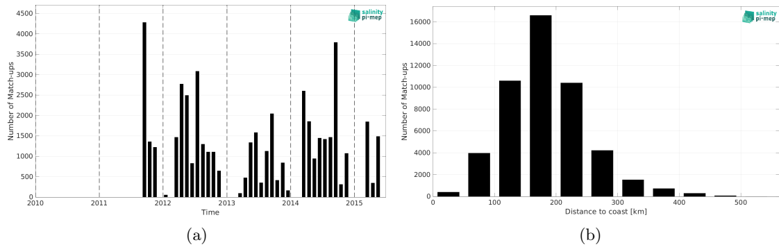
Figure 2: Number of match-ups between TSG (SAMOS) and Aquarius SSS L3 CAP v5 - Monthly (JPL) SSS as a function of time (a) and as function of the distance to coast (b) over the Gulf of Mexico Pi-MEP region and for the full satellite product period.
