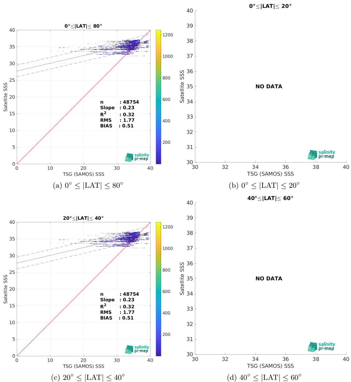
Figure 10: Contour maps of the concentration of Aquarius SSS L3 CAP v5 - Monthly (JPL) SSS (y-axis) versus TSG (SAMOS) SSS (x-axis) at match-up pairs for different latitude bands. For each plot, the red line shows x=y . The black thin and dashed lines indicate a linear fit through the data cloud and the \pm 95\% confidence levels, respectively. The number match-up pairs n , the slope and R^2 coefficient of the linear fit, the root mean square (RMS) and the mean bias between satellite and in situ data are indicated for each latitude band in each plots.
