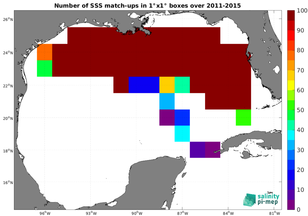
Figure 5: Number of SSS match-ups between TSG (SAMOS) SSS and the Aquarius SSS L3 CAP v5 - Monthly (JPL) SSS product for the Gulf of Mexico Pi-MEP region over 1°×1° boxes and for the full satellite product period.
