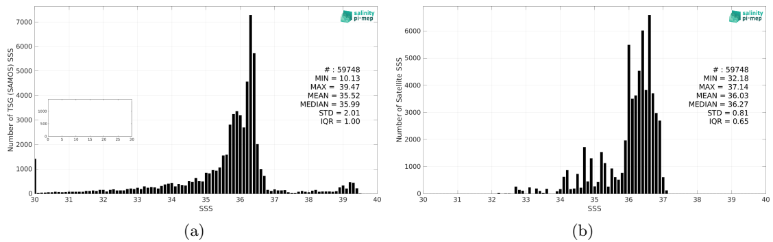
Figure 2: Histograms of SSS from TSG (SAMOS) (a) and Aquarius SSS L3 CAP v5 - Monthly (JPL) (b) considering all match-up pairs per bins of 0.1 over the Gulf of Mexico Pi-MEP region and for the full satellite product period.
