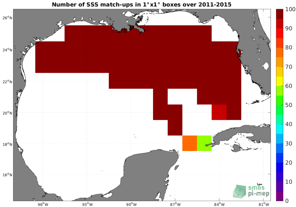
Figure 4: Number of SSS match-ups between TSG (SAMOS) SSS and the Aquarius SSS L3 CAP v5 - Monthly (JPL) SSS product for the Gulf of Mexico Pi-MEP region over 1^\circ \times 1^\circ boxes and for the full satellite product period.
