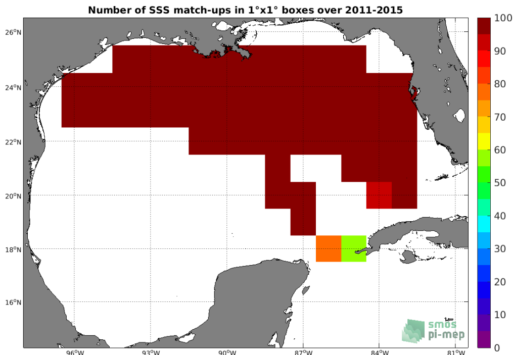
Figure 4: Number of SSS match-ups between TSG (SAMOS) SSS and the Aquarius SSS L3 CAP v5 - Monthly (JPL) SSS product for the Gulf of Mexico Pi-MEP region over 1°x1° boxes and for the full satellite product period.
