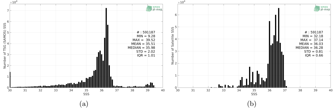
Figure 2: Histograms of SSS from TSG (SAMOS) (a) and Aquarius SSS L3 CAP v5 - Monthly (JPL) (b) considering all match-up pairs per bins of 0.1 over the Gulf of Mexico Pi-MEP region and for the full satellite product period.
