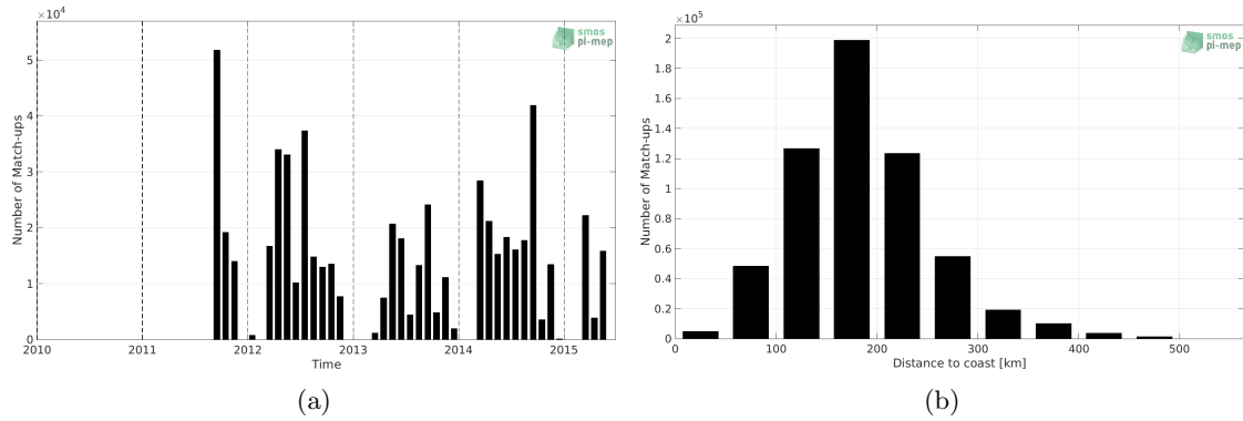
Figure 1: Number of match-ups between TSG (SAMOS) and Aquarius SSS L3 CAP v5 - Monthly (JPL) SSS as a function of time (a) and as function of the distance to coast (b) over the Gulf of Mexico Pi-MEP region and for the full satellite product period.
