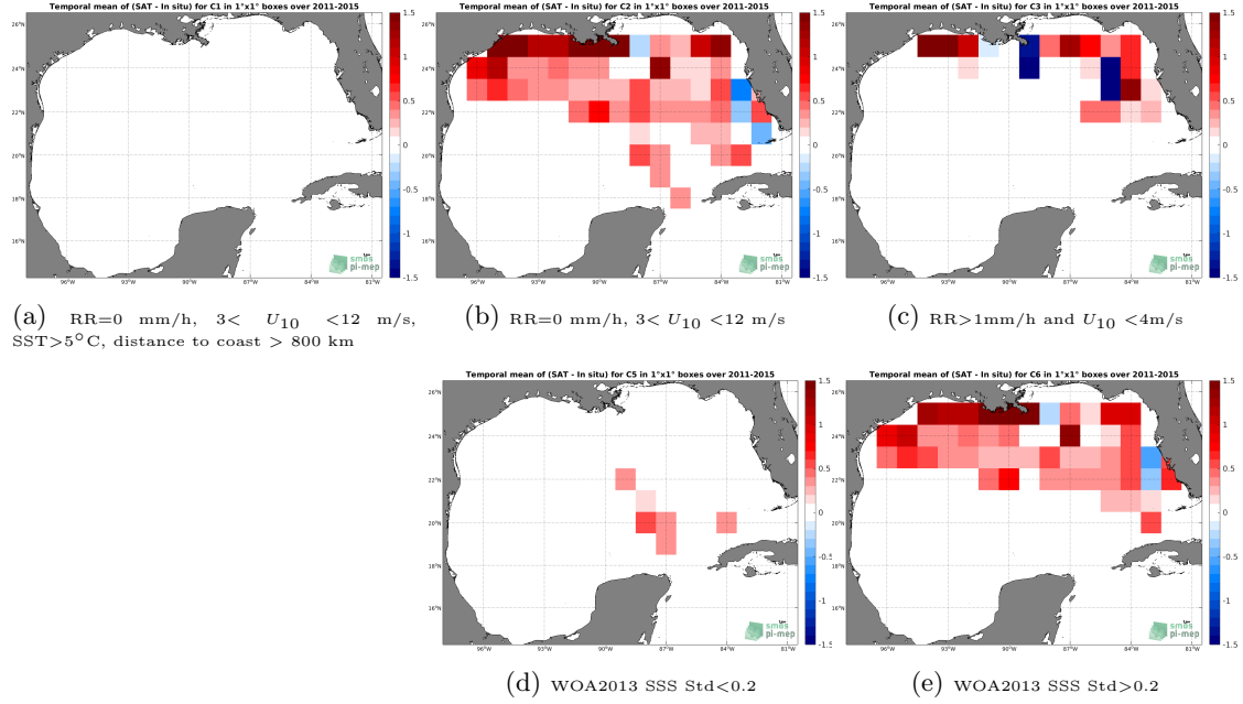
Figure 12: Temporal mean gridded over spatial boxes of size 1^{\circ}\times 1^{\circ} of \Delta\text{SSS} (Aquarius SSS L3 CAP v5 - Monthly (JPL) - TSG (SAMOS)) for 5 different subdatasets corresponding to: RR=0 mm/h, 3 < U_{10} < 12 m/s, SST > 5^{\circ}\text{C} , distance to coast > 800 km (a), RR=0 mm/h, 3 < U_{10} < 12 m/s (b), RR > 1 mm/h and U_{10} < 4 m/s (c), WOA2013 SSS Std < 0.2 (d), WOA2013 SSS Std > 0.2 (e).
