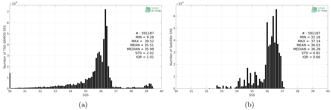
Figure 2: Histograms of SSS from TSG-SAMOS (a) and Aquarius-L3-JPL-V5-MONTHLY (b) considering all match-up pairs per bins of 0.1 over the Gulf of Mexico Pi-MEP region and for the full satellite product period.
