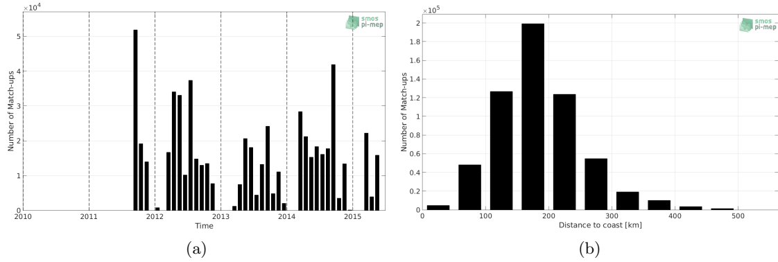
Figure 1: Number of match-ups between TSG-SAMOS and Aquarius-L3-JPL-V5-MONTHLY SSS as a function of time (a) and as function of the distance to coast (b) over the Gulf of Mexico Pi-MEP region and for the full satellite product period.
