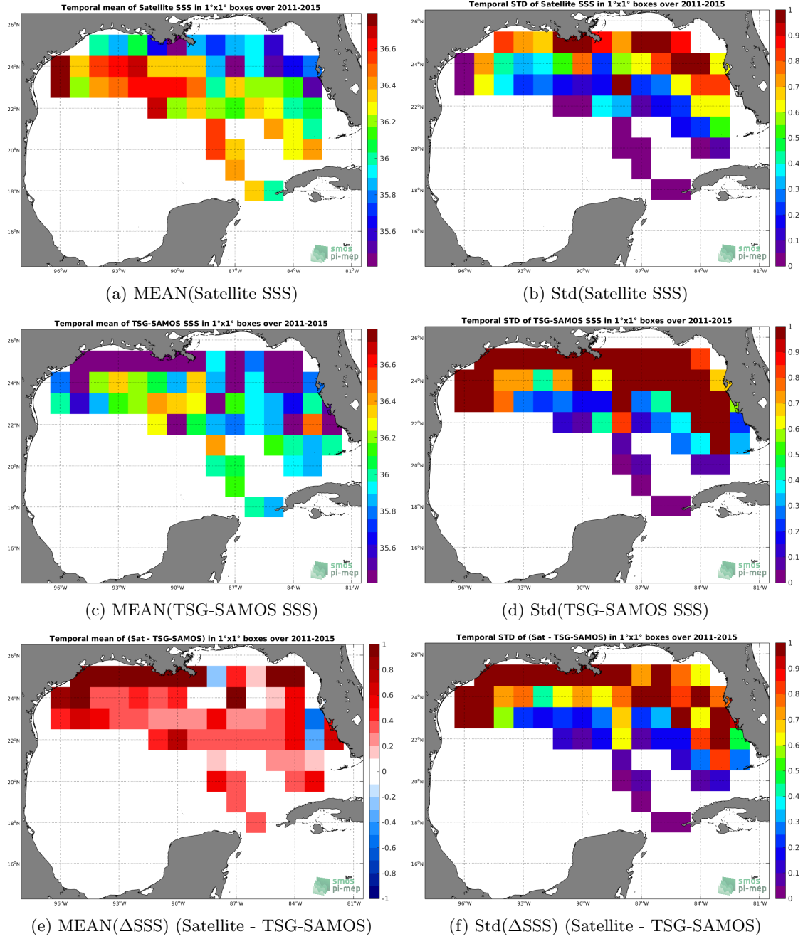
Figure 6: Temporal mean (left) and Std (right) of SSS from Aquarius-L3-JPL-V5-MONTHLY (top), TSG-SAMOS (middle), and of \Delta SSS (Satellite - TSG-SAMOS). Only match-up pairs are used to generate these maps.
