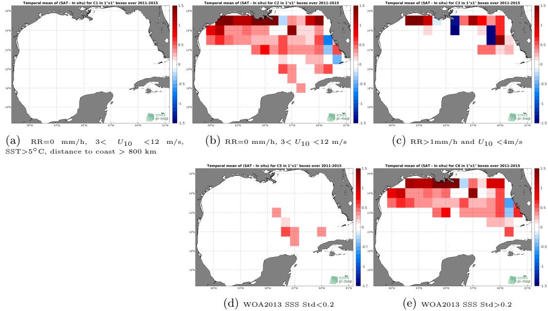
Figure 12: Temporal mean gridded over spatial boxes of size 1^{\circ}\times 1^{\circ} of \Delta\text{SSS} (Aquarius-L3-JPL-V5-MONTHLY - TSG-SAMOS) for 5 different subdatasets corresponding to: \text{RR}=0 mm/h, 3 < U_{10} < 12 m/s, \text{SST} > 5^{\circ}\text{C} , distance to coast > 800 km (a), \text{RR}=0 mm/h, 3 < U_{10} < 12 m/s (b), \text{RR} > 1 mm/h and U_{10} < 4 m/s (c), WOA2013 SSS Std < 0.2 (d), WOA2013 SSS Std > 0.2 (e).
