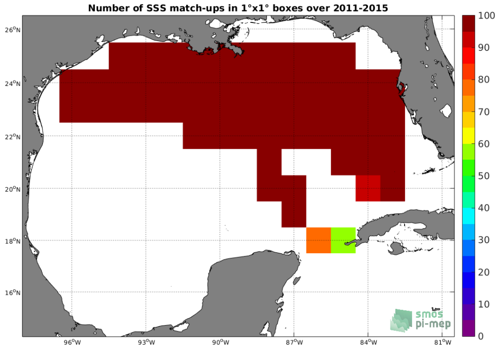
Figure 4: Number of SSS match-ups between TSG-SAMOS SSS and the Aquarius-L3-JPL-V5-MONTHLY SSS product for the Gulf of Mexico Pi-MEP region over 1^\circ \times 1^\circ boxes and for the full satellite product period.
