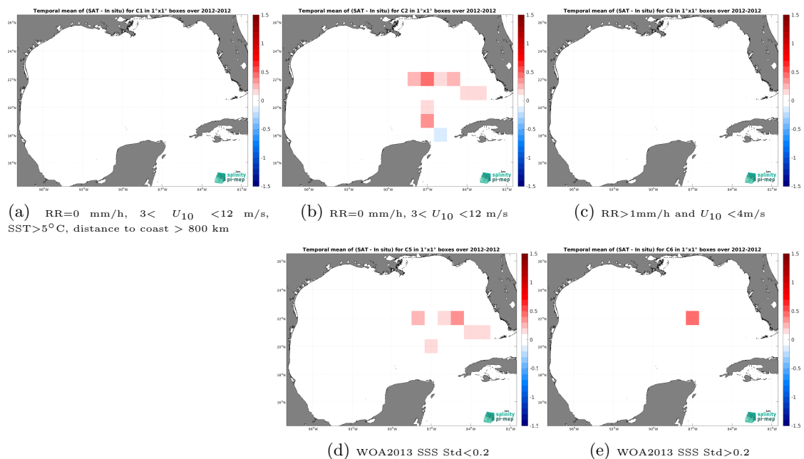
Figure 14: Temporal mean gridded over spatial boxes of size 1^\circ \times 1^\circ of \Delta SSS (Aquarius SSS L3 CAP v5 - Monthly (JPL) - TSG (GOSUD-Sailing-ship)) for 5 different subdatasets corresponding to:RR=0 mm/h, 3 < U_{10} < 12 m/s, SST >5^\circ C, distance to coast > 800 km (a), RR=0 mm/h, 3 < U_{10} < 12 m/s (b), RR >1 mm/h and U_{10} < 4 m/s (c), WOA2013 SSS Std <0.2 (d), WOA2013 SSS Std >0.2 (e).
