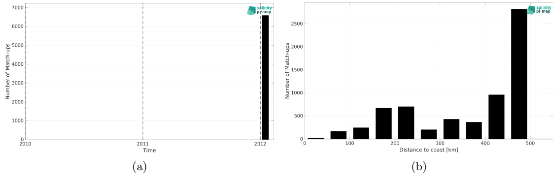
Figure 2: Number of match-ups between TSG (GOSUD-Sailing-ship) and Aquarius SSS L3 CAP v5 - Monthly (JPL) SSS as a function of time (a) and as function of the distance to coast (b) over the Gulf of Mexico Pi-MEP region and for the full satellite product period.
