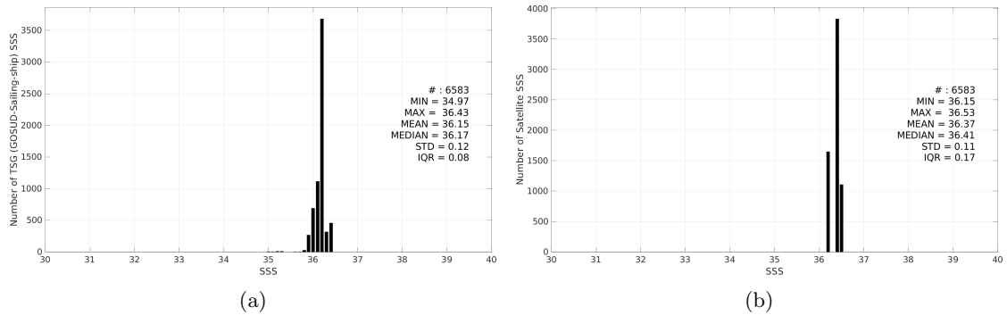
Figure 3: Histograms of SSS from TSG (GOSUD-Sailing-ship) (a) and Aquarius SSS L3 CAP v5 - Monthly (JPL) (b) considering all match-up pairs per bins of 0.1 over the Gulf of Mexico Pi-MEP region and for the full satellite product period.
