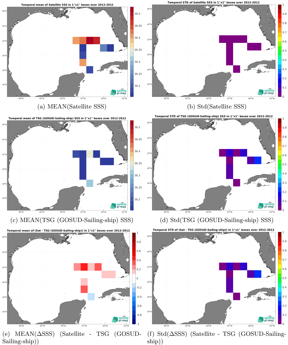
Figure 7: Temporal mean (left) and Std (right) of SSS from Aquarius SSS L3 CAP v5 - Monthly (JPL) (top), TSG (GOSUD-Sailing-ship) (middle), and of \Delta SSS (Satellite - TSG (GOSUD-Sailing-ship)). Only match-up pairs are used to generate these maps.
