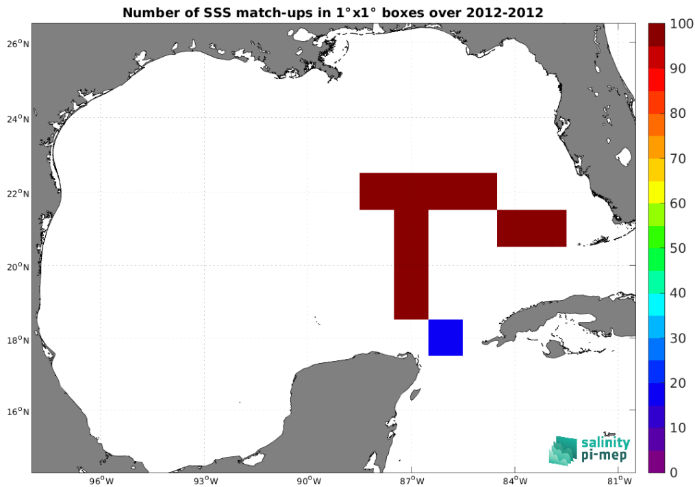
Figure 5: Number of SSS match-ups between TSG (GOSUD-Sailing-ship) SSS and the Aquarius SSS L3 CAP v5 - Monthly (JPL) SSS product for the Gulf of Mexico Pi-MEP region over 1^\circ \times 1^\circ boxes and for the full satellite product period.
