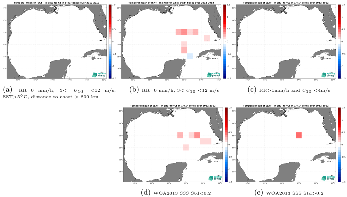
Figure 12: Temporal mean gridded over spatial boxes of size 1^{\circ}\times 1^{\circ} of \Delta SSS (Aquarius SSS L3 CAP v5 - Monthly (JPL) - TSG (GOSUD-Sailing-ship)) for 5 different subdatasets corresponding to:RR=0 mm/h, 3 < U_{10} < 12 m/s, SST >5^{\circ}\text{C} , distance to coast > 800 km (a), RR=0 mm/h, 3 < U_{10} < 12 m/s (b), RR >1 mm/h and U_{10} < 4 m/s (c), WOA2013 SSS Std <0.2 (d), WOA2013 SSS Std >0.2 (e).
