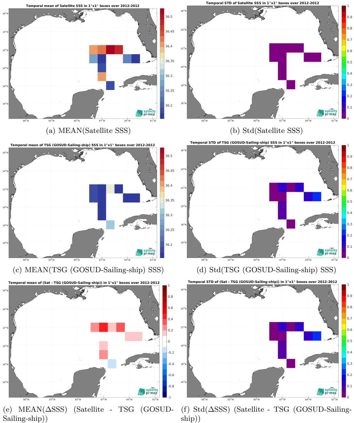
Figure 6: Temporal mean (left) and Std (right) of SSS from Aquarius SSS L3 CAP v5 - Monthly (JPL) (top), TSG (GOSUD-Sailing-ship) (middle), and of \Delta SSS (Satellite - TSG (GOSUD-Sailing-ship)). Only match-up pairs are used to generate these maps.
