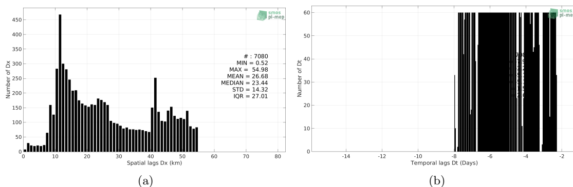
Figure 5: Histograms of the spatial (a) and temporal (b) lags between the time of the TSG (GOSUD-Sailing-ship) measurements and the date of the corresponding Aquarius SSS L3 CAP v5 - Monthly (JPL) SSS product.
