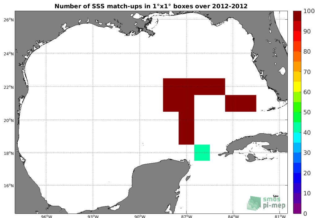
Figure 4: Number of SSS match-ups between TSG (GOSUD-Sailing-ship) SSS and the Aquarius SSS L3 CAP v5 - Monthly (JPL) SSS product for the Gulf of Mexico Pi-MEP region over 1^\circ \times 1^\circ boxes and for the full satellite product period.
