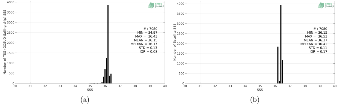
Figure 2: Histograms of SSS from TSG (GOSUD-Sailing-ship) (a) and Aquarius SSS L3 CAP v5 - Monthly (JPL) (b) considering all match-up pairs per bins of 0.1 over the Gulf of Mexico Pi-MEP region and for the full satellite product period.
