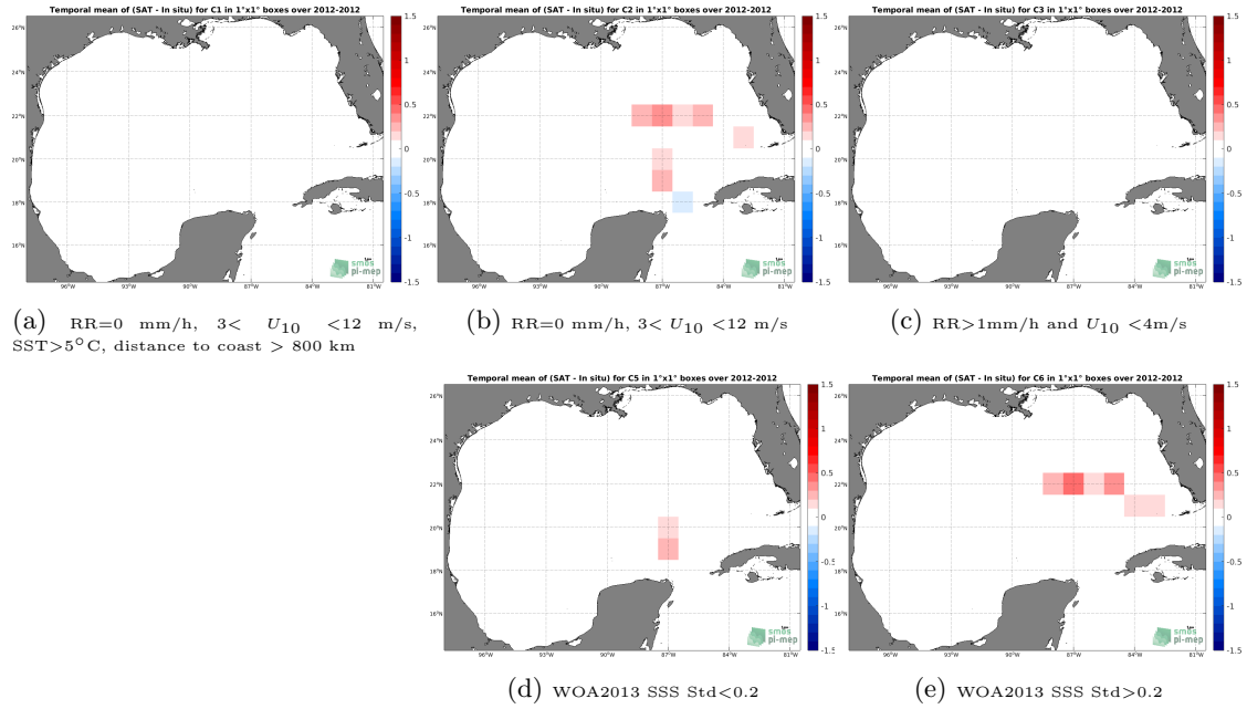
Figure 12: Temporal mean gridded over spatial boxes of size 1^\circ \times 1^\circ of \Delta SSS (Aquarius SSS L3 CAP v5 - Monthly (JPL) - TSG (GOSUD-Sailing-ship)) for 5 different subdatasets corresponding to: RR=0 mm/h, 3 < U_{10} < 12 m/s, SST >5^\circ\text{C} , distance to coast > 800 km (a), RR=0 mm/h, 3 < U_{10} < 12 m/s (b), RR >1 mm/h and U_{10} < 4 m/s (c), WOA2013 SSS Std <0.2 (d), WOA2013 SSS Std >0.2 (e).
