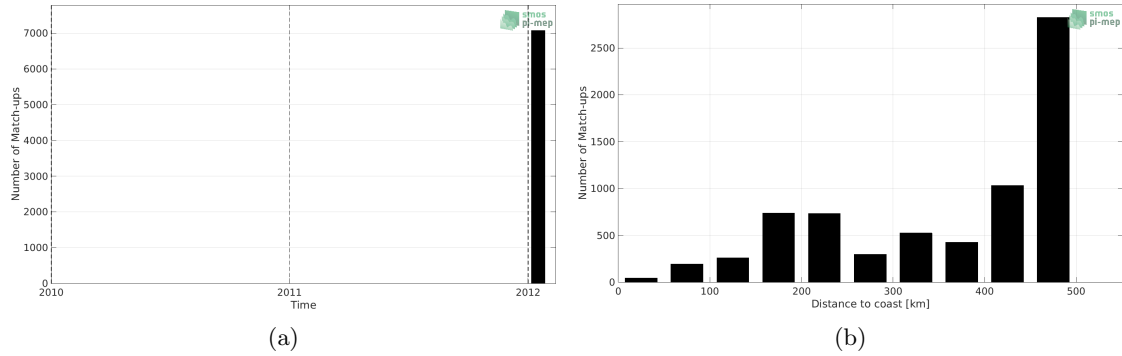
Figure 1: Number of match-ups between TSG (GOSUD-Sailing-ship) and Aquarius SSS L3 CAP v5 - Monthly (JPL) SSS as a function of time (a) and as function of the distance to coast (b) over the Gulf of Mexico Pi-MEP region and for the full satellite product period.
