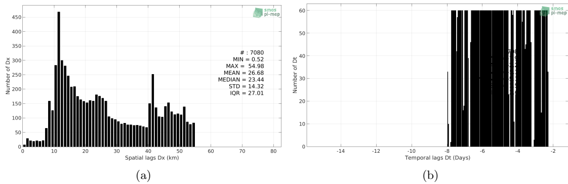
Figure 5: Histograms of the spatial (a) and temporal (b) lags between the time of the TSG-GOSUD-Sailing-ship measurements and the date of the corresponding Aquarius-L3-JPL-V5-MONTHLY SSS product.
