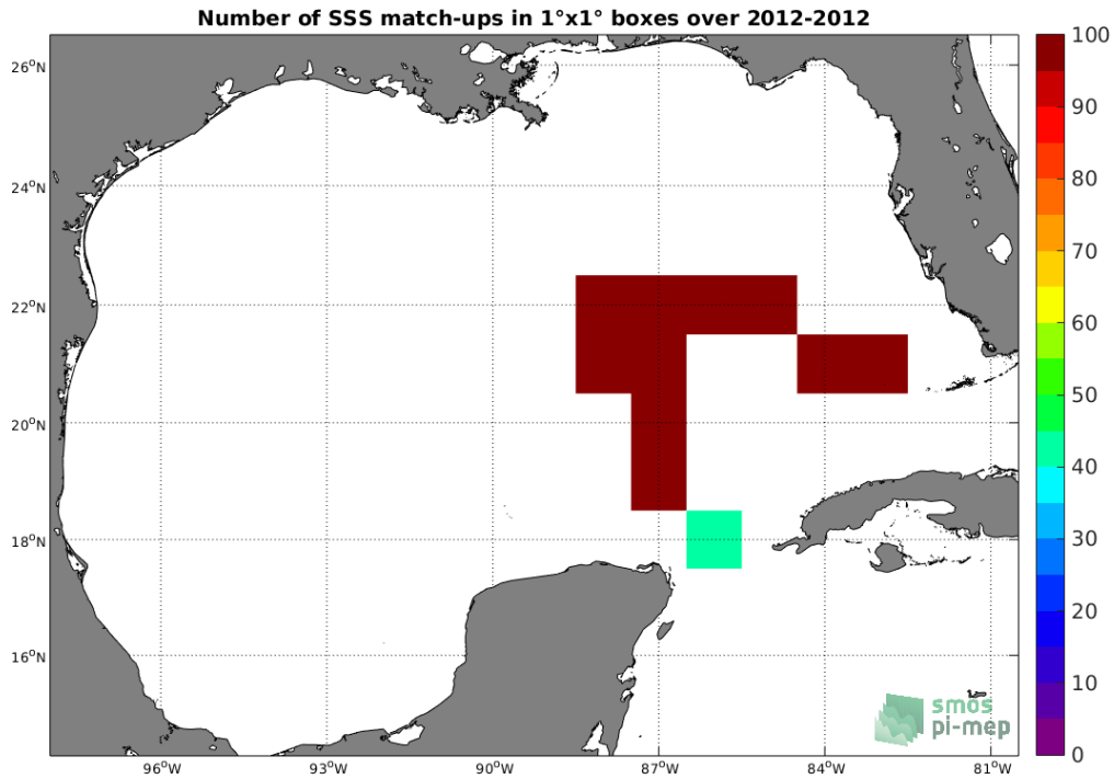
Figure 4: Number of SSS match-ups between TSG-GOSUD-Sailing-ship SSS and the Aquarius-L3-JPL-V5-MONTHLY SSS product for the Gulf of Mexico Pi-MEP region over 1^\circ \times 1^\circ boxes and for the full satellite product period.
