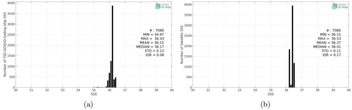
Figure 2: Histograms of SSS from TSG-GOSUD-Sailing-ship (a) and Aquarius-L3-JPL-V5-MONTHLY (b) considering all match-up pairs per bins of 0.1 over the Gulf of Mexico Pi-MEP region and for the full satellite product period.
