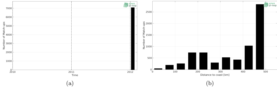
Figure 1: Number of match-ups between TSG-GOSUD-Sailing-ship and Aquarius-L3-JPL-V5-MONTHLY SSS as a function of time (a) and as function of the distance to coast (b) over the Gulf of Mexico Pi-MEP region and for the full satellite product period.
