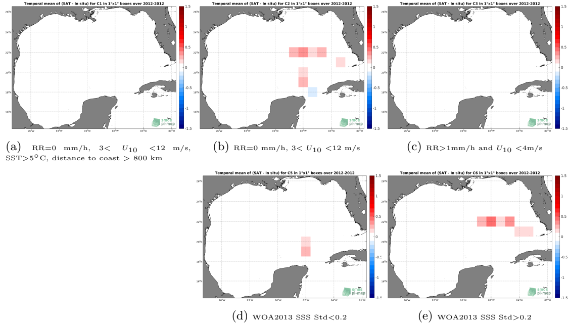
Figure 12: Temporal mean gridded over spatial boxes of size 1^\circ \times 1^\circ of \Delta SSS (Aquarius-L3-JPL-V5-MONTHLY - TSG-GOSUD-Sailing-ship) for 5 different subdatasets corresponding to: RR=0 mm/h, 3 < U_{10} < 12 m/s, SST > 5^\circ\text{C} , distance to coast > 800 km (a), RR=0 mm/h, 3 < U_{10} < 12 m/s (b), RR > 1 mm/h and U_{10} < 4 m/s (c), WOA2013 SSS Std < 0.2 (d), WOA2013 SSS Std > 0.2 (e).
