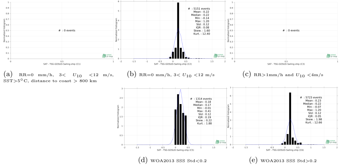
Figure 13: Normalized histogram of \Delta\text{SSS} (Aquarius-L3-JPL-V5-MONTHLY - TSG-GOSUD-Sailing-ship) for 5 different subdatasets corresponding to: RR=0 mm/h, 3 < U_{10} < 12 m/s, SST > 5^\circ\text{C} , distance to coast > 800 km (a), RR=0 mm/h, 3 < U_{10} < 12 m/s (b), RR > 1\text{mm/h} and U_{10} < 4\text{m/s} (c), WOA2013 SSS Std <0.2 (d), WOA2013 SSS Std >0.2 (e).
