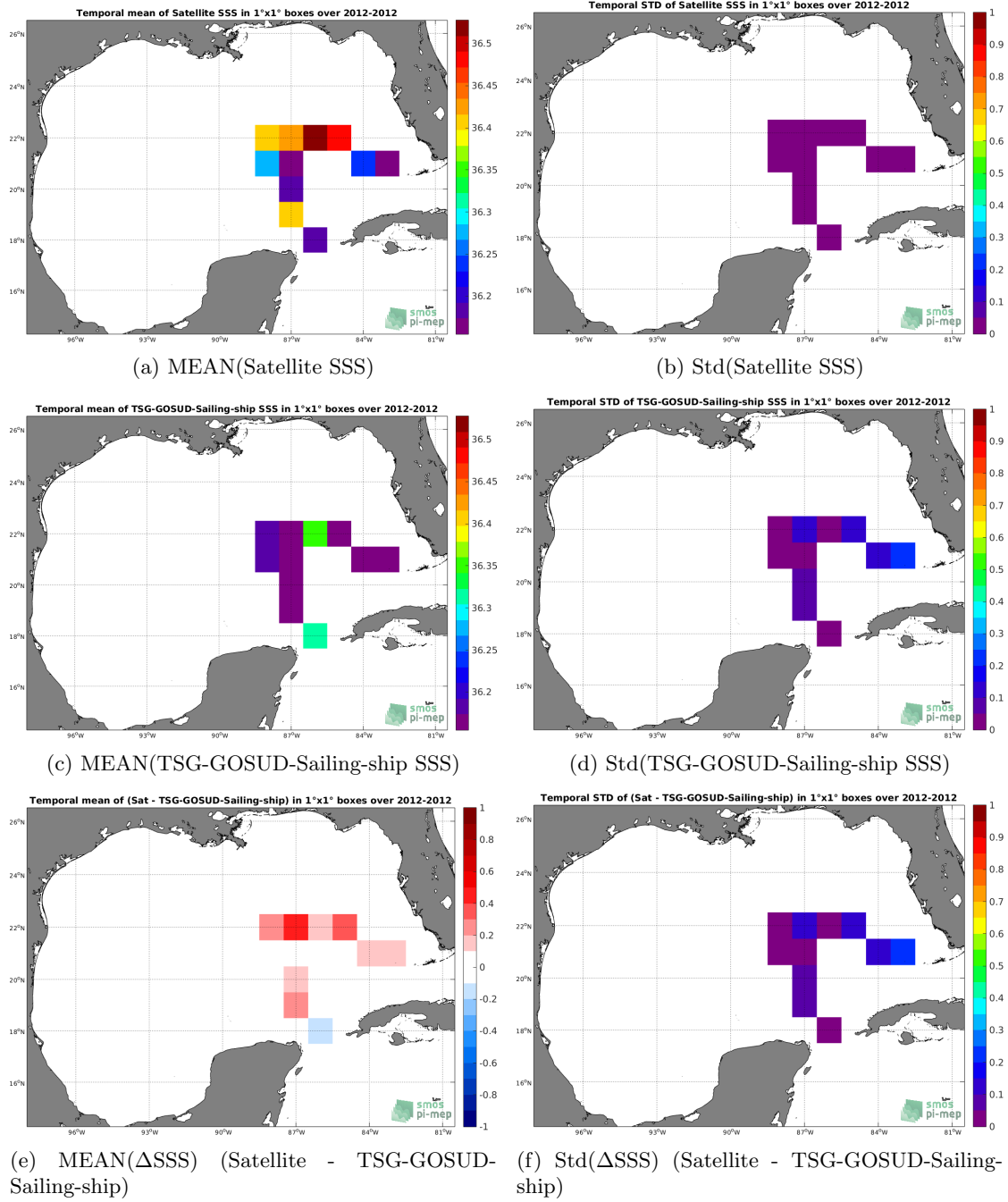
Figure 6: Temporal mean (left) and Std (right) of SSS from Aquarius-L3-JPL-V5-MONTHLY (top), TSG-GOSUD-Sailing-ship (middle), and of \Delta SSS (Satellite - TSG-GOSUD-Sailing-ship). Only match-up pairs are used to generate these maps.
