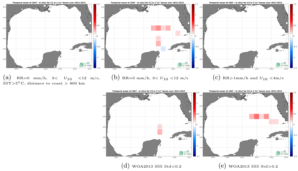
Figure 12: Temporal mean gridded over spatial boxes of size 1^\circ \times 1^\circ of \Delta SSS (Aquarius-L3-JPL-V5-MONTHLY - TSG-GOSUD-Sailing-ship) for 5 different subdatasets corresponding to:RR=0 mm/h, 3 < U_{10} < 12 m/s, SST >5^\circ\text{C} , distance to coast > 800 km (a), RR=0 mm/h, 3 < U_{10} < 12 m/s (b), RR >1 mm/h and U_{10} < 4 m/s (c), WOA2013 SSS Std <0.2 (d), WOA2013 SSS Std >0.2 (e).
