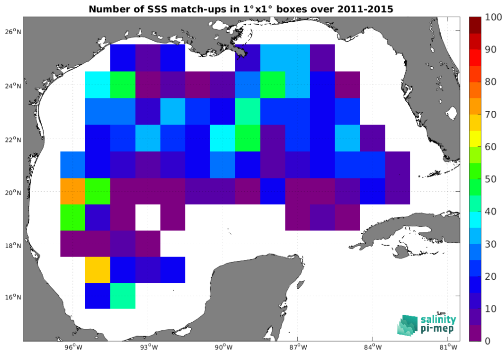
Figure 5: Number of SSS match-ups between Argo SSS and the Aquarius SSS L3 CAP v5 - Monthly (JPL) SSS product for the Gulf of Mexico Pi-MEP region over 1^\circ \times 1^\circ boxes and for the full satellite product period.
