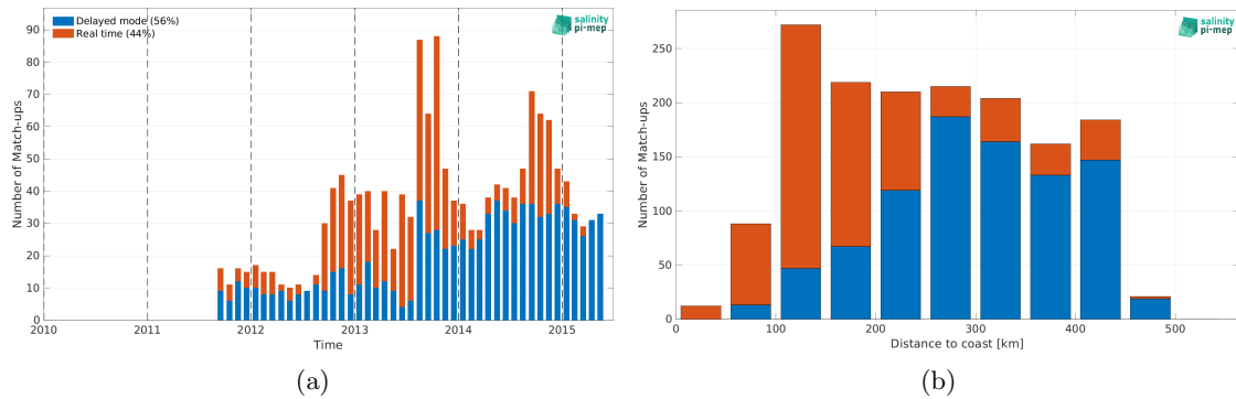
Figure 2: Number of match-ups between Argo and Aquarius SSS L3 CAP v5 - Monthly (JPL) SSS as a function of time (a) and as function of the distance to coast (b) over the Gulf of Mexico Pi-MEP region and for the full satellite product period.
