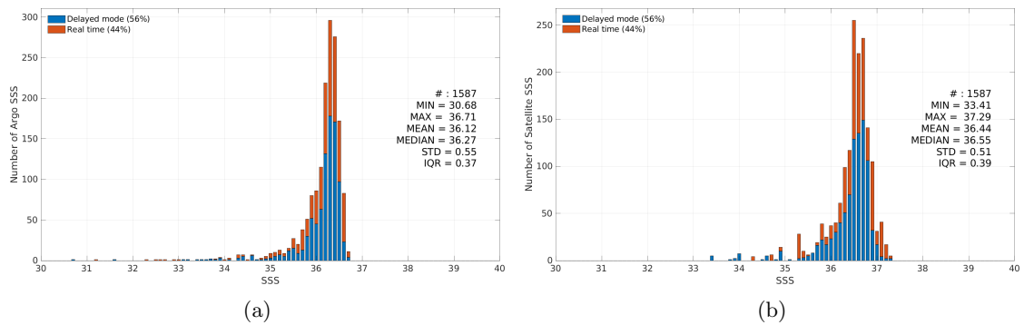
Figure 3: Histograms of SSS from Argo (a) and Aquarius SSS L3 CAP v5 - Monthly (JPL) (b) considering all match-up pairs per bins of 0.1 over the Gulf of Mexico Pi-MEP region and for the full satellite product period.
