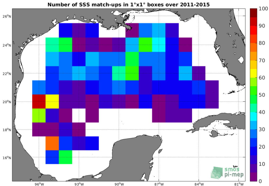
Figure 4: Number of SSS match-ups between Argo SSS and the Aquarius-L3-JPL-V5-MONTHLY SSS product for the Gulf of Mexico Pi-MEP region over 1^\circ \times 1^\circ boxes and for the full satellite product period.
