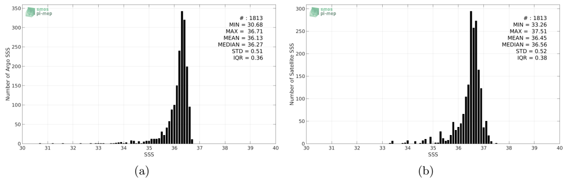
Figure 2: Histograms of SSS from Argo (a) and Aquarius-L3-JPL-V5-MONTHLY (b) considering all match-up pairs per bins of 0.1 over the Gulf of Mexico Pi-MEP region and for the full satellite product period.
