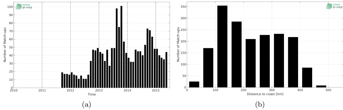
Figure 1: Number of match-ups between Argo and Aquarius-L3-JPL-V5-MONTHLY SSS as a function of time (a) and as function of the distance to coast (b) over the Gulf of Mexico Pi-MEP region and for the full satellite product period.
