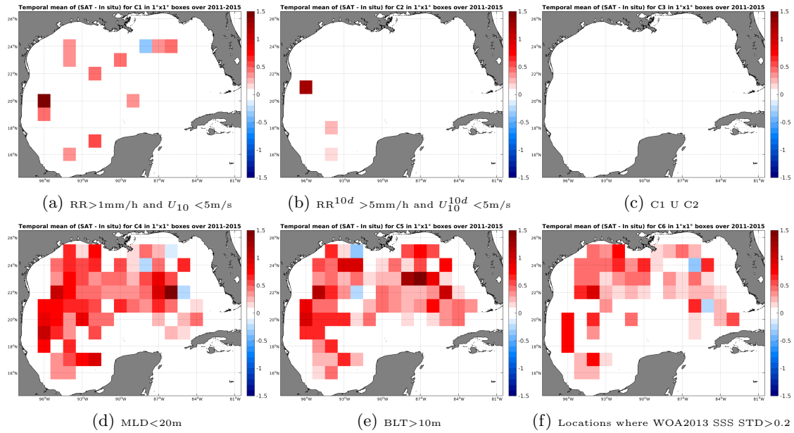
Figure 12: Temporal mean gridded over spatial boxes of size 1^\circ \times 1^\circ of \Delta SSS (Aquarius-L3-JPL-V4-MONTHLY - Argo) for 6 different subdatasets corresponding to:RR >1 mm/h and U_{10} < 5 m/s (a), RR 10d > 5 mm/h and U_{10}^{10d} < 5 m/s (b), C1 U C2 (c),MLD <20 m (d),BLT >10 m (e),Locations where WOA2013 SSS STD >0.2 (f).
