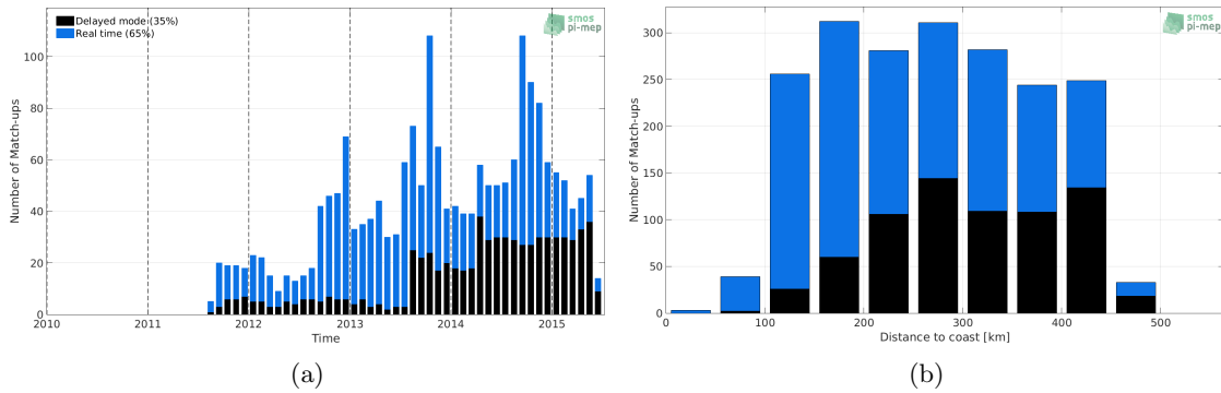
Figure 1: Number of match-ups between Argo and Aquarius SSS L2-AVERAGED OR v5 (NASA-GSFC) SSS as a function of time (a) and as function of the distance to coast (b) over the Gulf of Mexico Pi-MEP region and for the full satellite product period.
