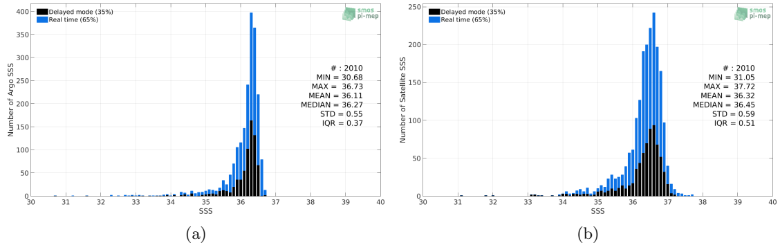
Figure 2: Histograms of SSS from Argos (a) and Aquarius SSS L2-AVERAGED OR v5 (NASA-GSFC) (b) considering all match-up pairs per bins of 0.1 over the Gulf of Mexico Pi-MEP region and for the full satellite product period.
