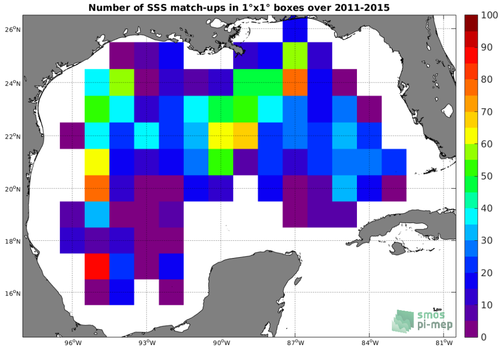
Figure 4: Number of SSS match-ups between Argo SSS and the Aquarius SSS L2-AVERAGED OR v5 (NASA-GSFC) SSS product for the Gulf of Mexico Pi-MEP region over 1^\circ \times 1^\circ boxes and for the full satellite product period.
