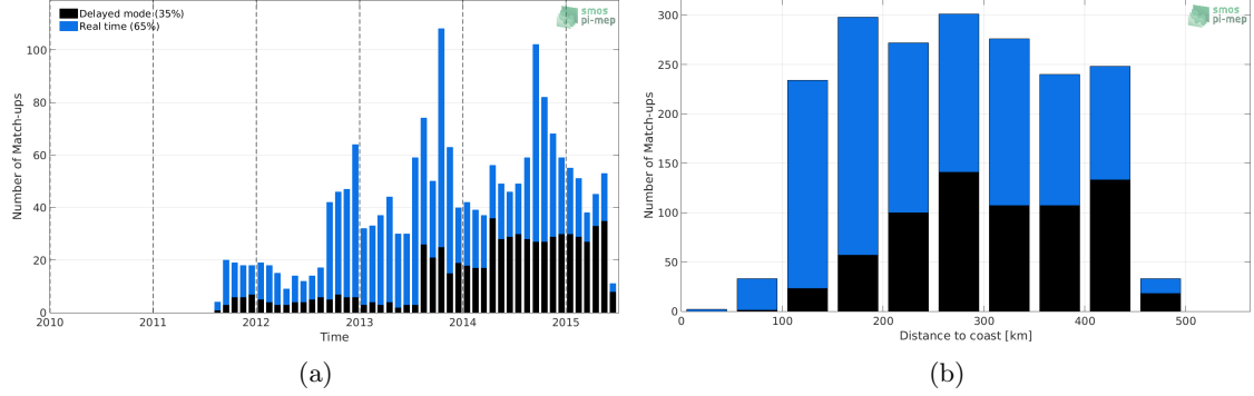
Figure 1: Number of match-ups between Argo and Aquarius SSS L2-AVERAGED CAP v5 (JPL) SSS as a function of time (a) and as function of the distance to coast (b) over the Gulf of Mexico Pi-MEP region and for the full satellite product period.
