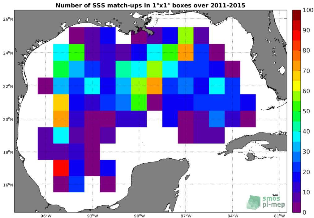
Figure 4: Number of SSS match-ups between Argo SSS and the Aquarius SSS L2-AVERAGED CAP v5 (JPL) SSS product for the Gulf of Mexico Pi-MEP region over 1°x1° boxes and for the full satellite product period.
