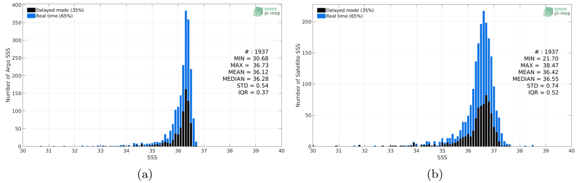
Figure 2: Histograms of SSS from Argo (a) and Aquarius SSS L2-AVERAGED CAP v5 (JPL) (b) considering all match-up pairs per bins of 0.1 over the Gulf of Mexico Pi-MEP region and for the full satellite product period.
