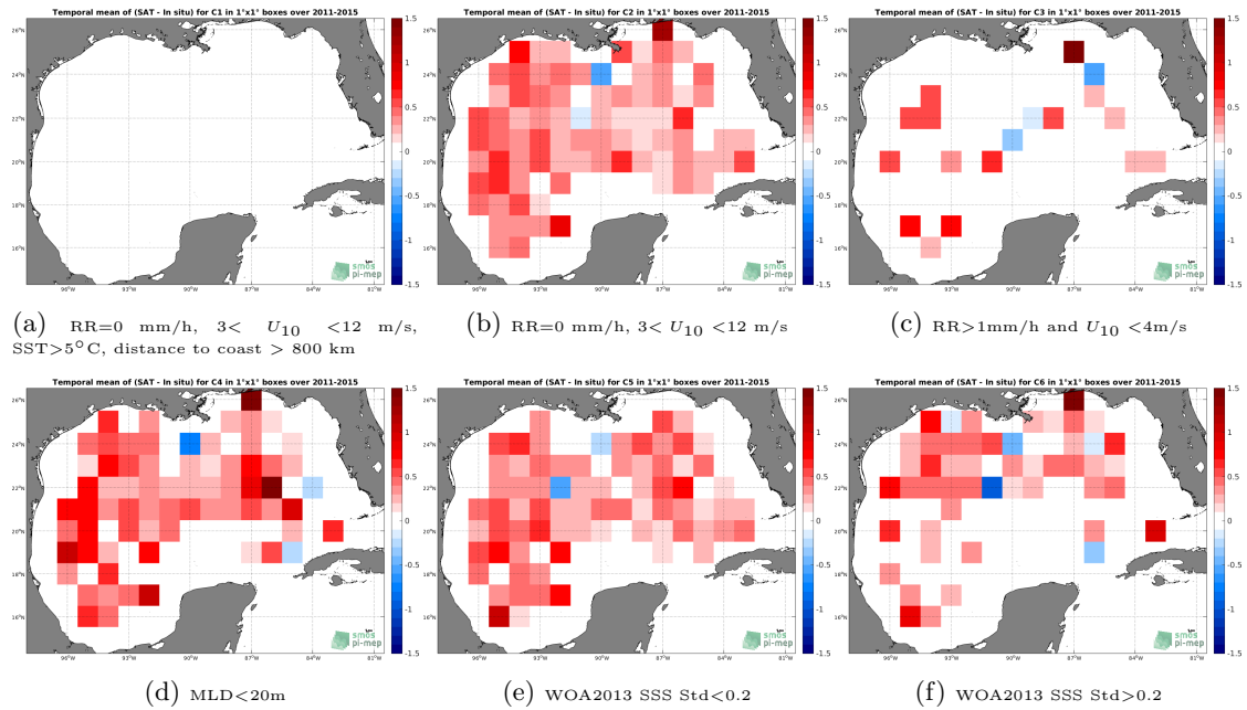
Figure 12: Temporal mean gridded over spatial boxes of size 1^\circ \times 1^\circ of \Delta SSS (Aquarius SSS L2-AVERAGED CAP v5 (JPL) - Argo) for 6 different subdatasets corresponding to:RR=0 mm/h, 3 < U_{10} < 12 m/s, SST > 5^\circ\text{C} , distance to coast > 800 km (a), RR=0 mm/h, 3 < U_{10} < 12 m/s (b), RR > 1 mm/h and U_{10} < 4 m/s (c),MLD < 20 m (d),WOA2013 SSS Std < 0.2 (e),WOA2013 SSS Std > 0.2 (f).
