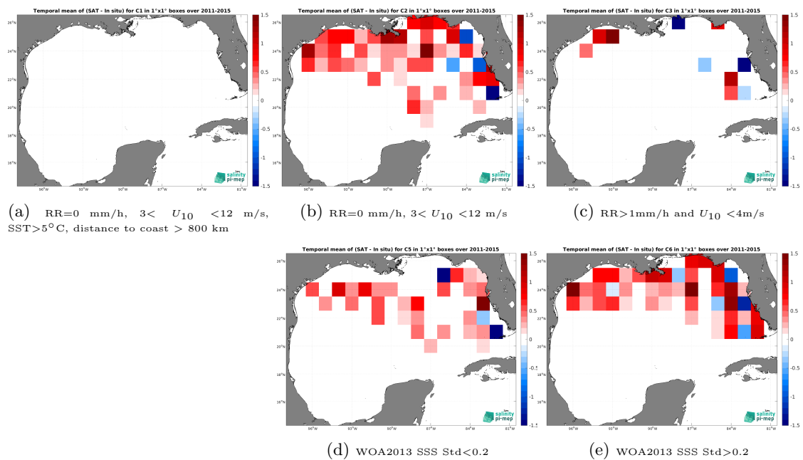
Figure 14: Temporal mean gridded over spatial boxes of size 1^\circ \times 1^\circ of \Delta SSS (Aquarius SSS L2 OR v5 (NASA-GSFC) - TSG (SAMOS)) for 5 different subdatasets corresponding to:RR=0 mm/h, 3 < U_{10} < 12 m/s, SST >5^\circ C, distance to coast > 800 km (a), RR=0 mm/h, 3 < U_{10} < 12 m/s (b), RR >1 mm/h and U_{10} < 4 m/s (c), WOA2013 SSS Std <0.2 (d), WOA2013 SSS Std >0.2 (e).
