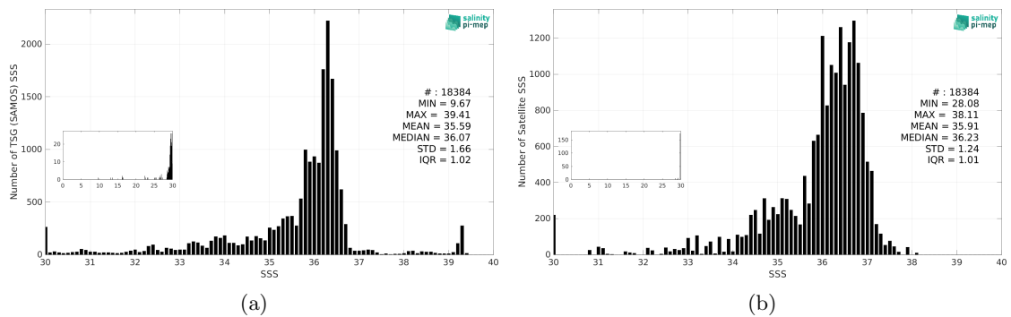
Figure 3: Histograms of SSS from TSG (SAMOS) (a) and Aquarius SSS L2 OR v5 (NASA-GSFC) (b) considering all match-up pairs per bins of 0.1 over the Gulf of Mexico Pi-MEP region and for the full satellite product period.
