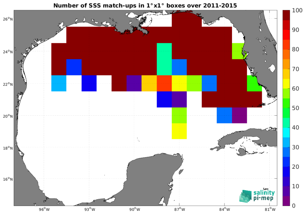
Figure 5: Number of SSS match-ups between TSG (SAMOS) SSS and the Aquarius SSS L2 OR v5 (NASA-GSFC) SSS product for the Gulf of Mexico Pi-MEP region over 1°×1° boxes and for the full satellite product period.
