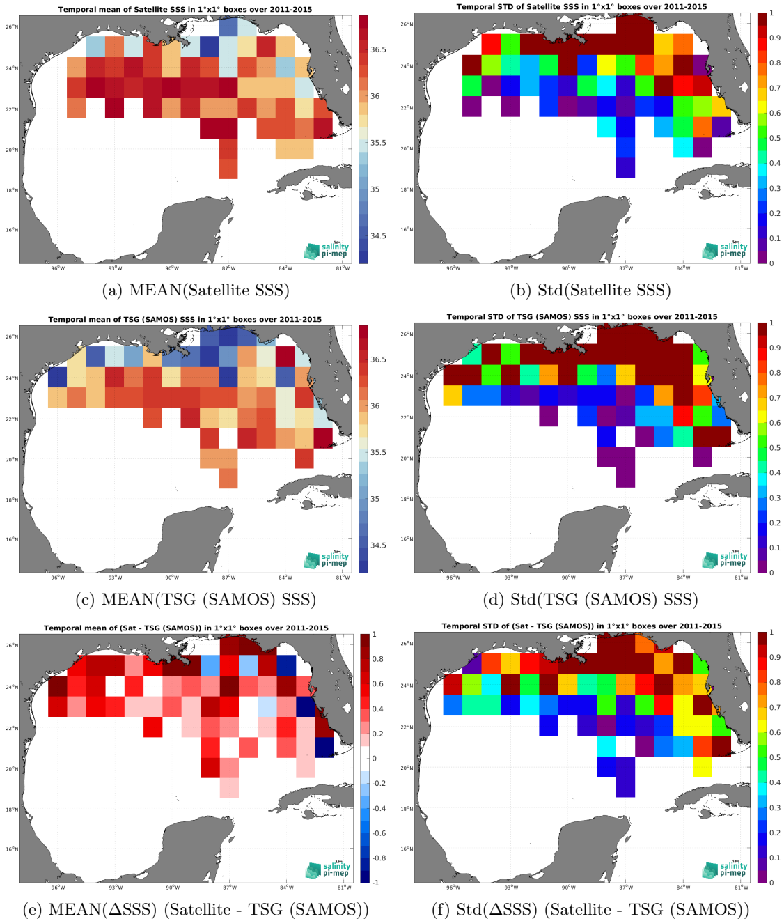
Figure 7: Temporal mean (left) and Std (right) of SSS from Aquarius SSS L2 OR v5 (NASA-GSFC) (top), TSG (SAMOS) (middle), and of \Delta SSS (Satellite - TSG (SAMOS)). Only match-up pairs are used to generate these maps.
