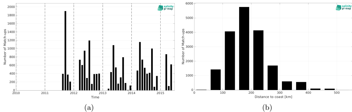
Figure 2: Number of match-ups between TSG (SAMOS) and Aquarius SSS L2 OR v5 (NASA-GSFC) SSS as a function of time (a) and as function of the distance to coast (b) over the Gulf of Mexico Pi-MEP region and for the full satellite product period.
