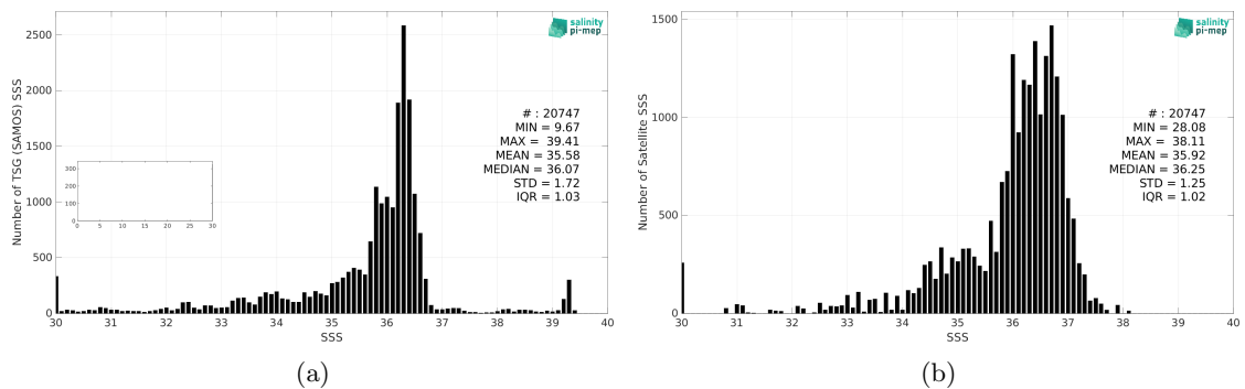
Figure 2: Histograms of SSS from TSG (SAMOS) (a) and Aquarius SSS L2 OR v5 (NASA-GSFC) (b) considering all match-up pairs per bins of 0.1 over the Gulf of Mexico Pi-MEP region and for the full satellite product period.
