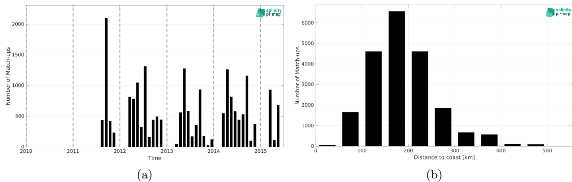
Figure 1: Number of match-ups between TSG (SAMOS) and Aquarius SSS L2 OR v5 (NASA-GSFC) SSS as a function of time (a) and as function of the distance to coast (b) over the Gulf of Mexico Pi-MEP region and for the full satellite product period.
