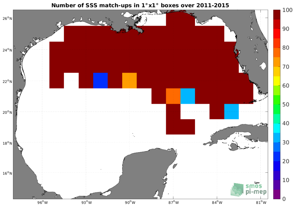
Figure 4: Number of SSS match-ups between TSG (SAMOS) SSS and the Aquarius SSS L2 OR v5 (NASA-GSFC) SSS product for the Gulf of Mexico Pi-MEP region over 1^\circ \times 1^\circ boxes and for the full satellite product period.
