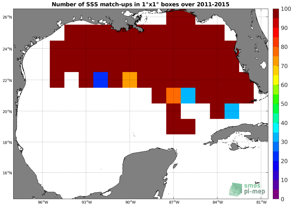
Figure 4: Number of SSS match-ups between TSG (SAMOS) SSS and the Aquarius SSS L2 OR v5 (NASA-GSFC) SSS product for the Gulf of Mexico Pi-MEP region over 1^{\circ} \times 1^{\circ} boxes and for the full satellite product period.
