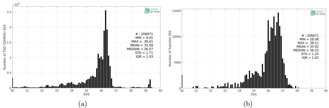
Figure 2: Histograms of SSS from TSG (SAMOS) (a) and Aquarius SSS L2 OR v5 (NASA-GSFC) (b) considering all match-up pairs per bins of 0.1 over the Gulf of Mexico Pi-MEP region and for the full satellite product period.
