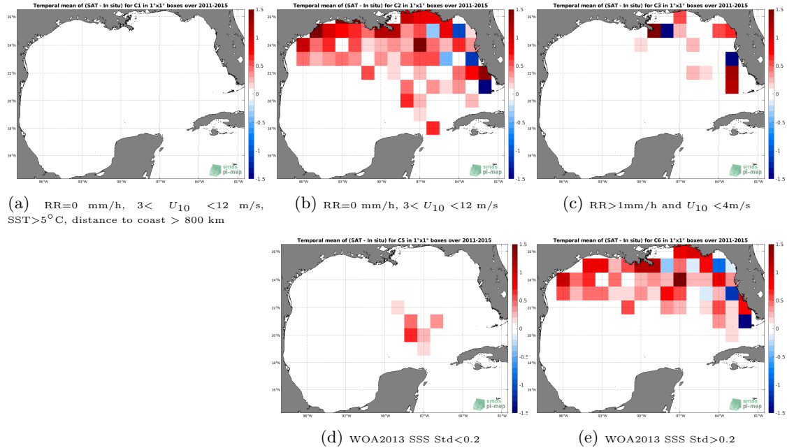
Figure 12: Temporal mean gridded over spatial boxes of size 1^{\circ}\times 1^{\circ} of \Delta\text{SSS} (Aquarius SSS L2 OR v5 (NASA-GSFC) - TSG (SAMOS)) for 5 different subdatasets corresponding to:RR=0 mm/h, 3 < U_{10} < 12 m/s, SST > 5^{\circ}\text{C} , distance to coast > 800 km (a), RR=0 mm/h, 3 < U_{10} < 12 m/s (b), RR > 1 mm/h and U_{10} < 4 m/s (c), WOA2013 SSS Std < 0.2 (d), WOA2013 SSS Std > 0.2 (e).
