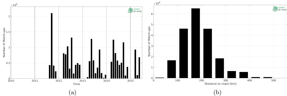
Figure 1: Number of match-ups between TSG (SAMOS) and Aquarius SSS L2 OR v5 (NASA-GSFC) SSS as a function of time (a) and as function of the distance to coast (b) over the Gulf of Mexico Pi-MEP region and for the full satellite product period.
