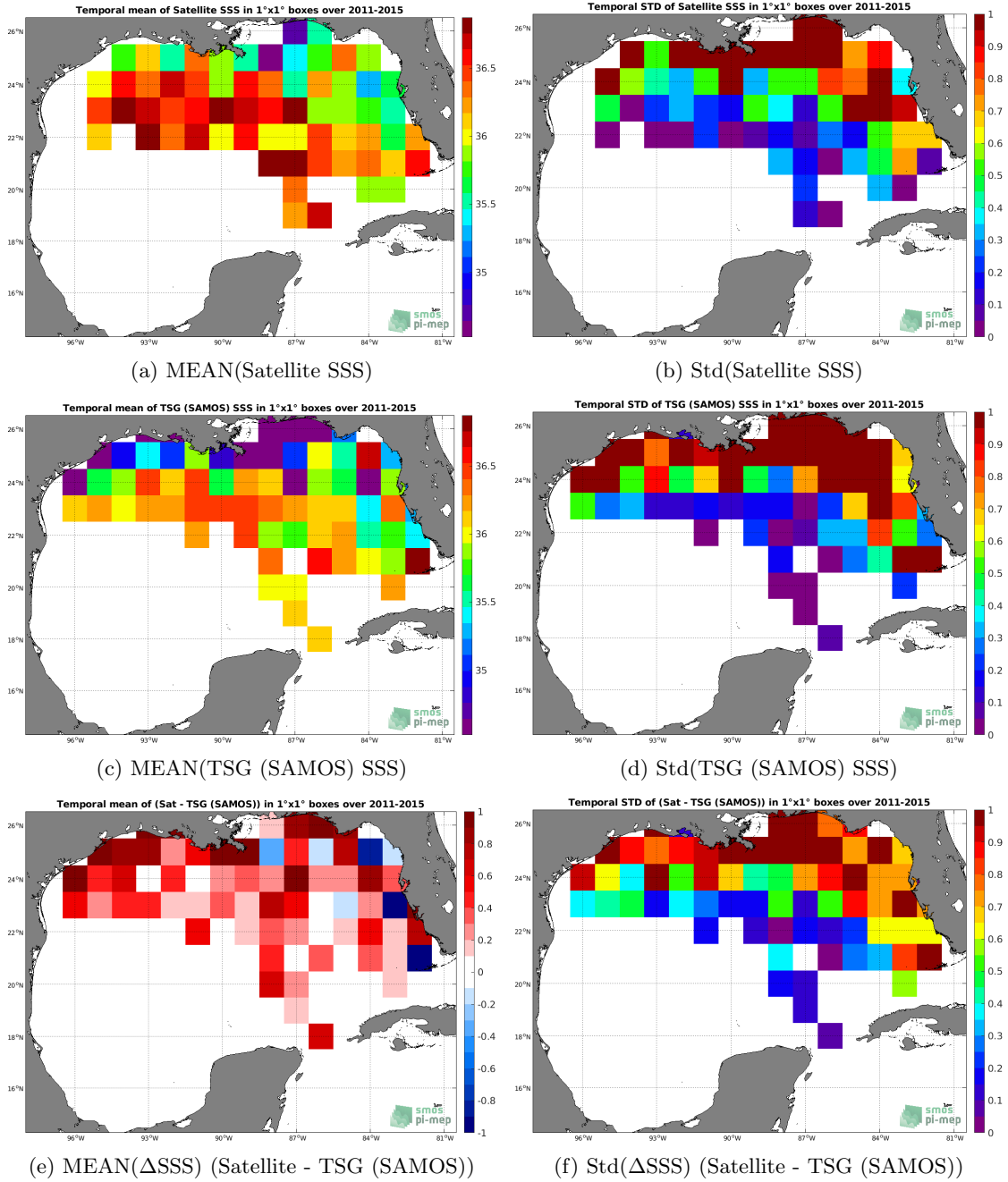
Figure 6: Temporal mean (left) and Std (right) of SSS from Aquarius SSS L2 OR v5 (NASA-GSFC) (top), TSG (SAMOS) (middle), and of \Delta SSS (Satellite - TSG (SAMOS)). Only match-up pairs are used to generate these maps.
