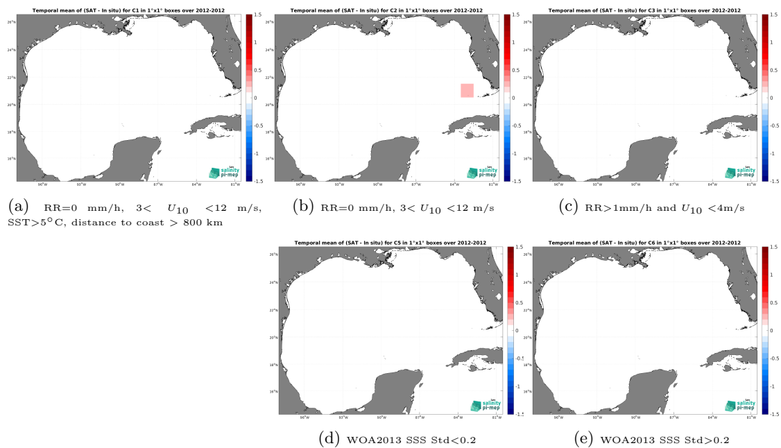
Figure 14: Temporal mean gridded over spatial boxes of size 1^\circ \times 1^\circ of \Delta SSS (Aquarius SSS L2 OR v5 (NASA-GSFC) - TSG (GOSUD-Sailing-ship)) for 5 different subdatasets corresponding to:RR=0 mm/h, 3 < U_{10} < 12 m/s, SST >5^\circ C, distance to coast > 800 km (a), RR=0 mm/h, 3 < U_{10} < 12 m/s (b), RR >1 mm/h and U_{10} < 4 m/s (c), WOA2013 SSS Std <0.2 (d), WOA2013 SSS Std >0.2 (e).
