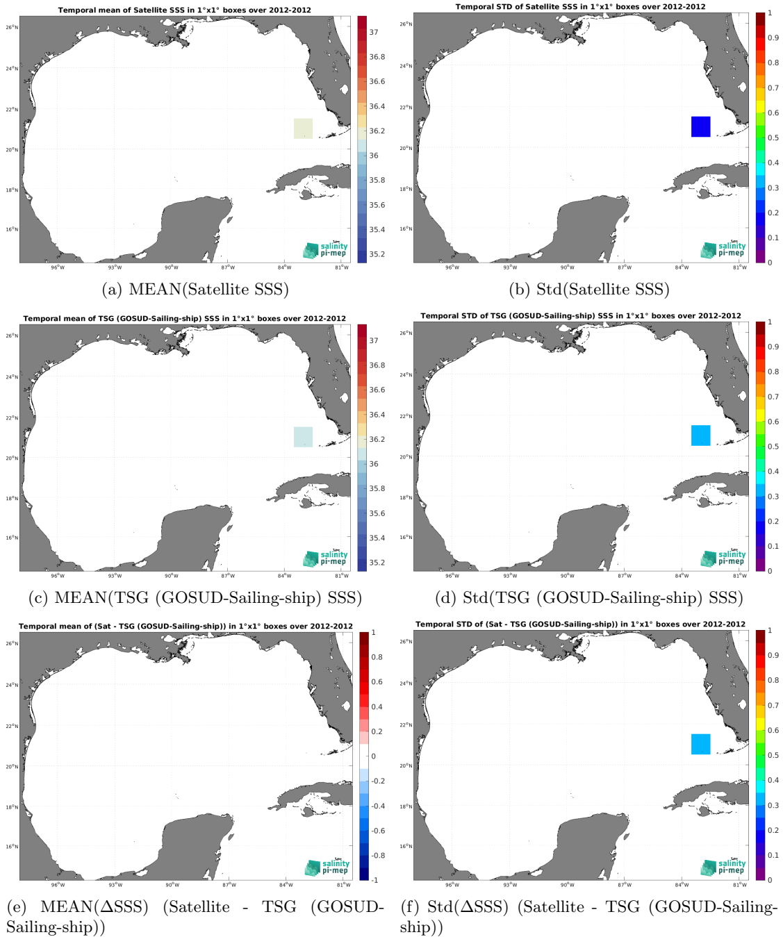
Figure 7: Temporal mean (left) and Std (right) of SSS from Aquarius SSS L2 OR v5 (NASA-GSFC) (top), TSG (GOSUD-Sailing-ship) (middle), and of \Delta SSS (Satellite - TSG (GOSUD-Sailing-ship)). Only match-up pairs are used to generate these maps.
