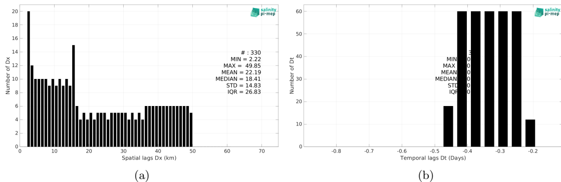
Figure 6: Histograms of the spatial (a) and temporal (b) lags between the location/time of the TSG (GOSUD-Sailing-ship) measurement and the date of the corresponding Aquarius SSS L2 OR v5 (NASA-GSFC) SSS pixel.
