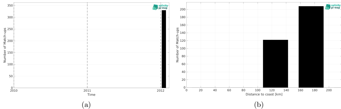
Figure 2: Number of match-ups between TSG (GOSUD-Sailing-ship) and Aquarius SSS L2 OR v5 (NASA-GSFC) SSS as a function of time (a) and as function of the distance to coast (b) over the Gulf of Mexico Pi-MEP region and for the full satellite product period.
