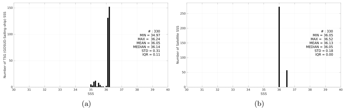
Figure 3: Histograms of SSS from TSG (GOSUD-Sailing-ship) (a) and Aquarius SSS L2 OR v5 (NASA-GSFC) (b) considering all match-up pairs per bins of 0.1 over the Gulf of Mexico Pi-MEP region and for the full satellite product period.
