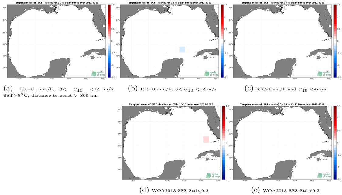
Figure 12: Temporal mean gridded over spatial boxes of size 1^\circ \times 1^\circ of \Delta SSS (Aquarius SSS L2 OR v5 (NASA-GSFC) - TSG (GOSUD-Sailing-ship)) for 5 different subdatasets corresponding to:RR=0 mm/h, 3 < U_{10} < 12 m/s, SST >5^\circ\text{C} , distance to coast > 800 km (a), RR=0 mm/h, 3 < U_{10} < 12 m/s (b), RR >1 mm/h and U_{10} < 4 m/s (c), WOA2013 SSS Std <0.2 (d), WOA2013 SSS Std >0.2 (e).
