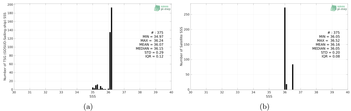
Figure 2: Histograms of SSS from TSG (GOSUD-Sailing-ship) (a) and Aquarius SSS L2 OR v5 (NASA-GSFC) (b) considering all match-up pairs per bins of 0.1 over the Gulf of Mexico Pi-MEP region and for the full satellite product period.
