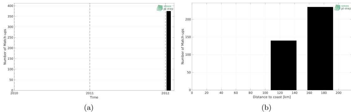
Figure 1: Number of match-ups between TSG (GOSUD-Sailing-ship) and Aquarius SSS L2 OR v5 (NASA-GSFC) SSS as a function of time (a) and as function of the distance to coast (b) over the Gulf of Mexico Pi-MEP region and for the full satellite product period.
