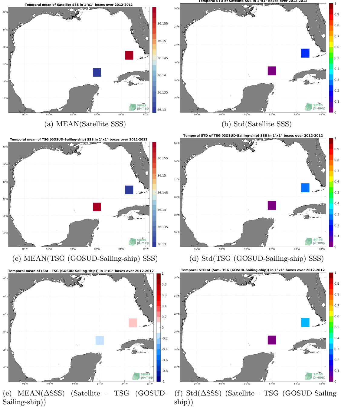
Figure 6: Temporal mean (left) and Std (right) of SSS from Aquarius SSS L2 OR v5 (NASA-GSFC) (top), TSG (GOSUD-Sailing-ship) (middle), and of \Delta SSS (Satellite - TSG (GOSUD-Sailing-ship)). Only match-up pairs are used to generate these maps.
