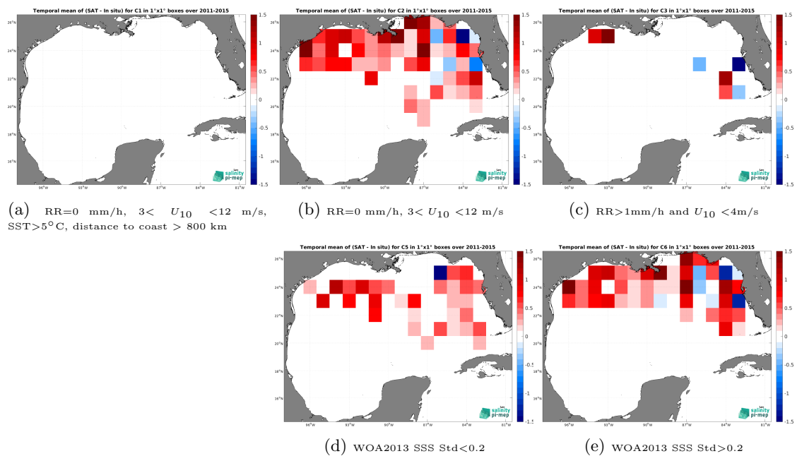
Figure 14: Temporal mean gridded over spatial boxes of size 1^\circ \times 1^\circ of \Delta\text{SSS} (Aquarius SSS L2 CAP v5 (JPL) - TSG (SAMOS)) for 5 different subdatasets corresponding to:RR=0 mm/h, 3 < U_{10} < 12 m/s, SST >5^\circ\text{C} , distance to coast > 800 km (a), RR=0 mm/h, 3 < U_{10} < 12 m/s (b), RR >1 mm/h and U_{10} < 4 m/s (c), WOA2013 SSS Std <0.2 (d), WOA2013 SSS Std >0.2 (e).
