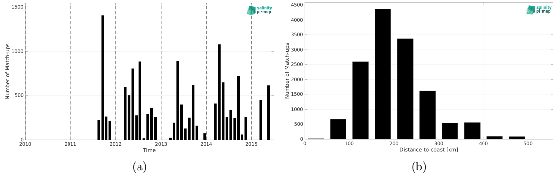
Figure 2: Number of match-ups between TSG (SAMOS) and Aquarius SSS L2 CAP v5 (JPL) SSS as a function of time (a) and as function of the distance to coast (b) over the Gulf of Mexico Pi-MEP region and for the full satellite product period.
