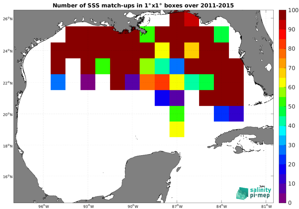
Figure 5: Number of SSS match-ups between TSG (SAMOS) SSS and the Aquarius SSS L2 CAP v5 (JPL) SSS product for the Gulf of Mexico Pi-MEP region over 1°×1° boxes and for the full satellite product period.
