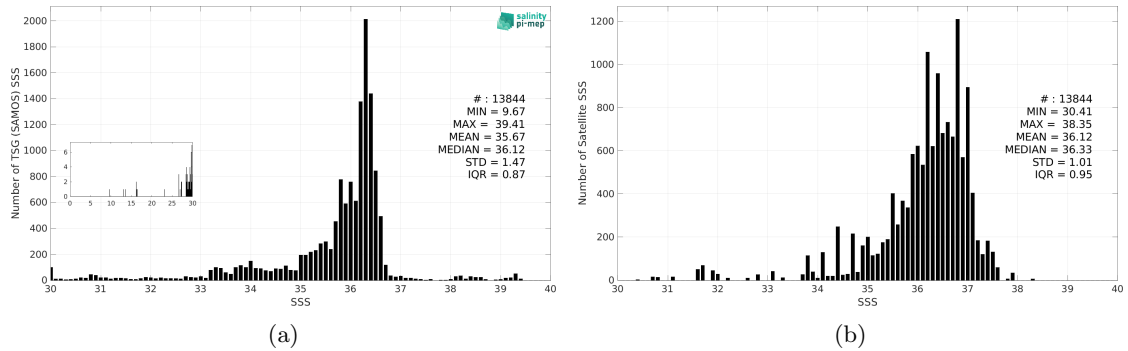
Figure 3: Histograms of SSS from TSG (SAMOS) (a) and Aquarius SSS L2 CAP v5 (JPL) (b) considering all match-up pairs per bins of 0.1 over the Gulf of Mexico Pi-MEP region and for the full satellite product period.
