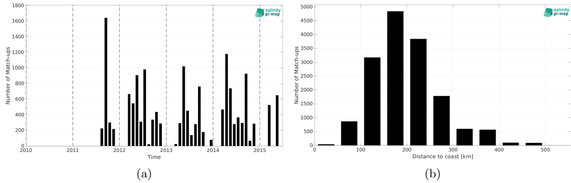
Figure 1: Number of match-ups between TSG (SAMOS) and Aquarius SSS L2 CAP v5 (JPL) SSS as a function of time (a) and as function of the distance to coast (b) over the Gulf of Mexico Pi-MEP region and for the full satellite product period.
