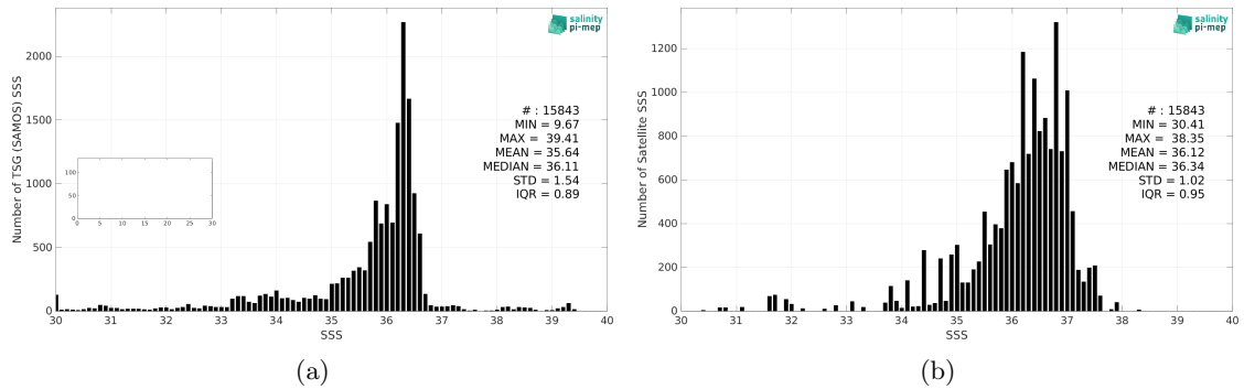
Figure 2: Histograms of SSS from TSG (SAMOS) (a) and Aquarius SSS L2 CAP v5 (JPL) (b) considering all match-up pairs per bins of 0.1 over the Gulf of Mexico Pi-MEP region and for the full satellite product period.
