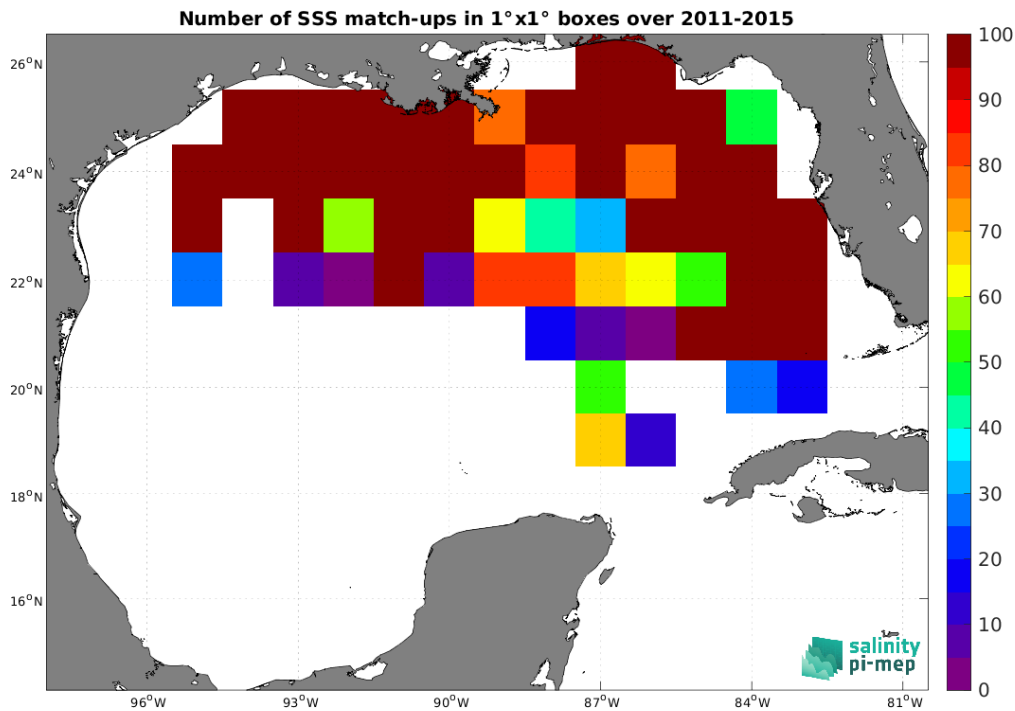
Figure 4: Number of SSS match-ups between TSG (SAMOS) SSS and the Aquarius SSS L2 CAP v5 (JPL) SSS product for the Gulf of Mexico Pi-MEP region over 1°×1° boxes and for the full satellite product period.
