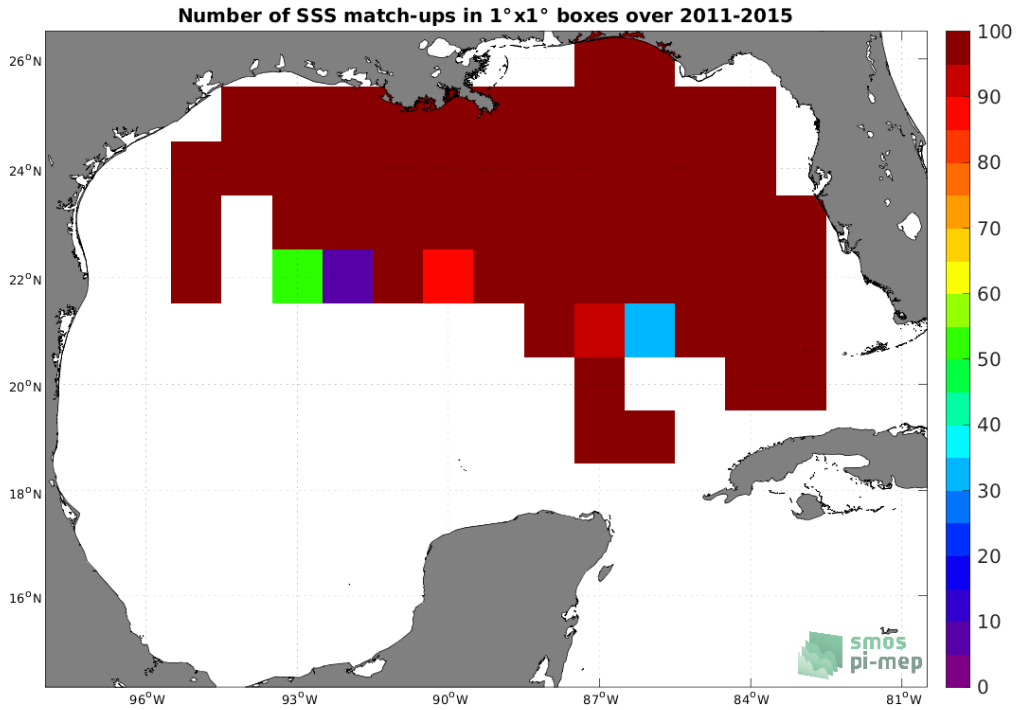
Figure 4: Number of SSS match-ups between TSG (SAMOS) SSS and the Aquarius SSS L2 CAP v5 (JPL) SSS product for the Gulf of Mexico Pi-MEP region over 1^\circ \times 1^\circ boxes and for the full satellite product period.
