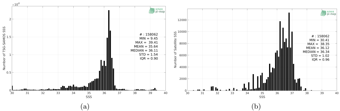
Figure 2: Histograms of SSS from TSG-SAMOS (a) and Aquarius-L2-JPL-V5 (b) considering all match-up pairs per bins of 0.1 over the Gulf of Mexico Pi-MEP region and for the full satellite product period.
