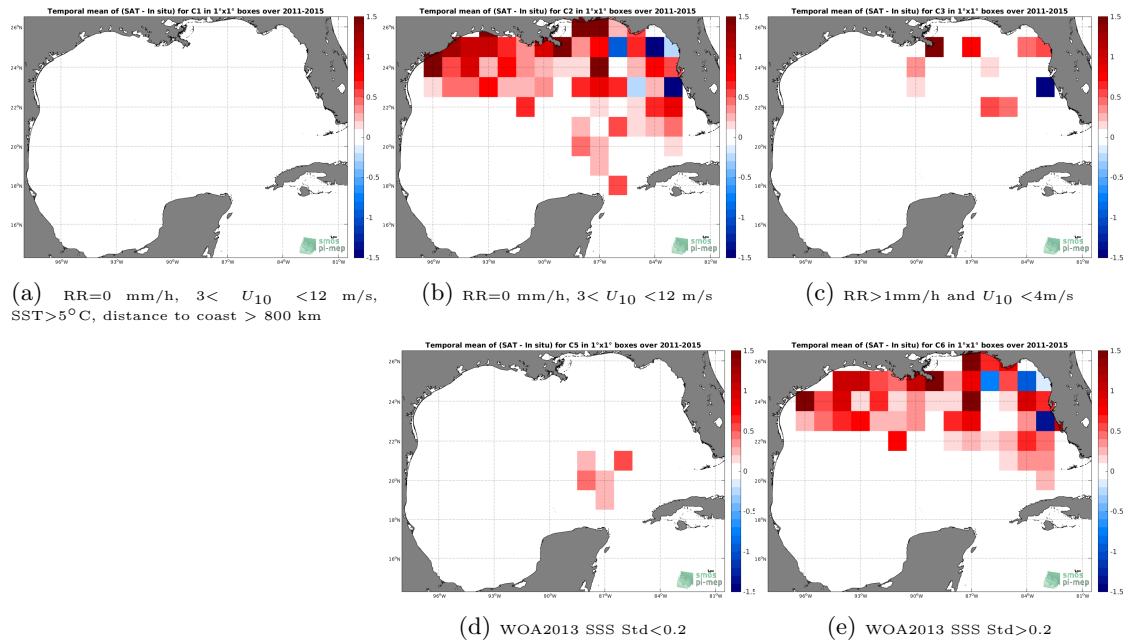
Figure 12: Temporal mean gridded over spatial boxes of size 1^{\circ}\times 1^{\circ} of \Delta\text{SSS} (Aquarius-L2-JPL-V5 - TSG-SAMOS) for 5 different subdatasets corresponding to:RR=0 mm/h, 3 < U_{10} < 12 m/s, SST >5^{\circ}\text{C} , distance to coast > 800 km (a), RR=0 mm/h, 3 < U_{10} < 12 m/s (b), RR >1 mm/h and U_{10} < 4 m/s (c), WOA2013 SSS Std <0.2 (d), WOA2013 SSS Std >0.2 (e).
