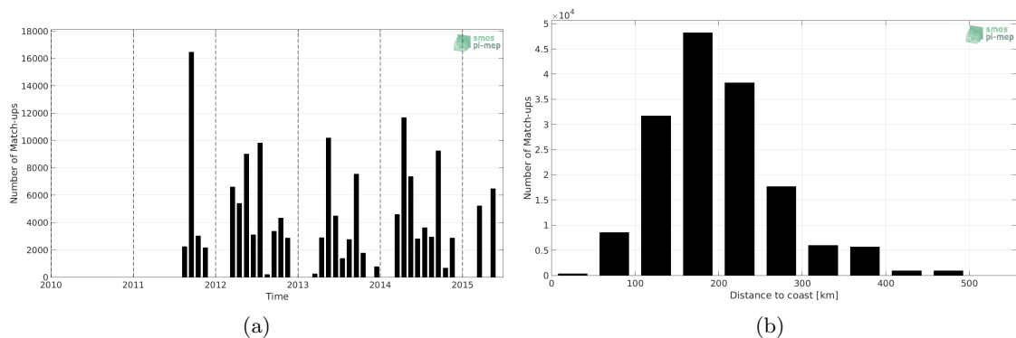
Figure 1: Number of match-ups between TSG-SAMOS and Aquarius-L2-JPL-V5 SSS as a function of time (a) and as function of the distance to coast (b) over the Gulf of Mexico Pi-MEP region and for the full satellite product period.
