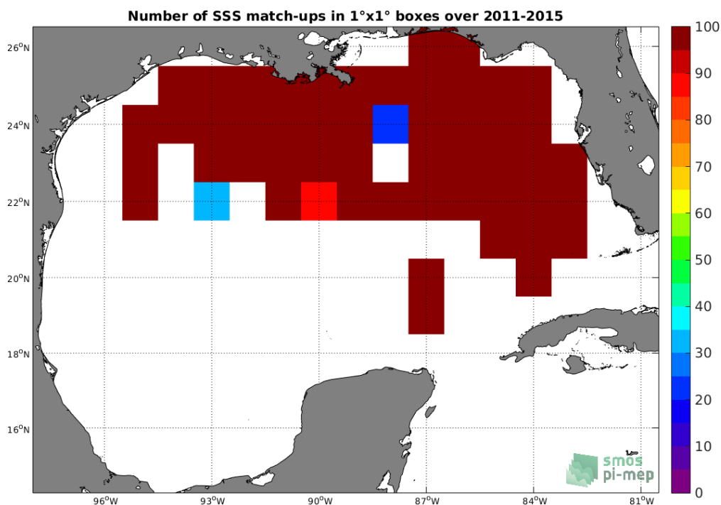
Figure 4: Number of SSS match-ups between TSG-SAMOS SSS and the Aquarius-L2-JPL-V5 SSS product for the Gulf of Mexico Pi-MEP region over 1^\circ \times 1^\circ boxes and for the full satellite product period.
