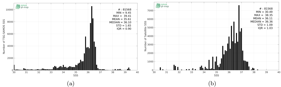
Figure 2: Histograms of SSS from TSG-SAMOS (a) and Aquarius-L2-JPL-V5 (b) considering all match-up pairs per bins of 0.1 over the Gulf of Mexico Pi-MEP region and for the full satellite product period.
