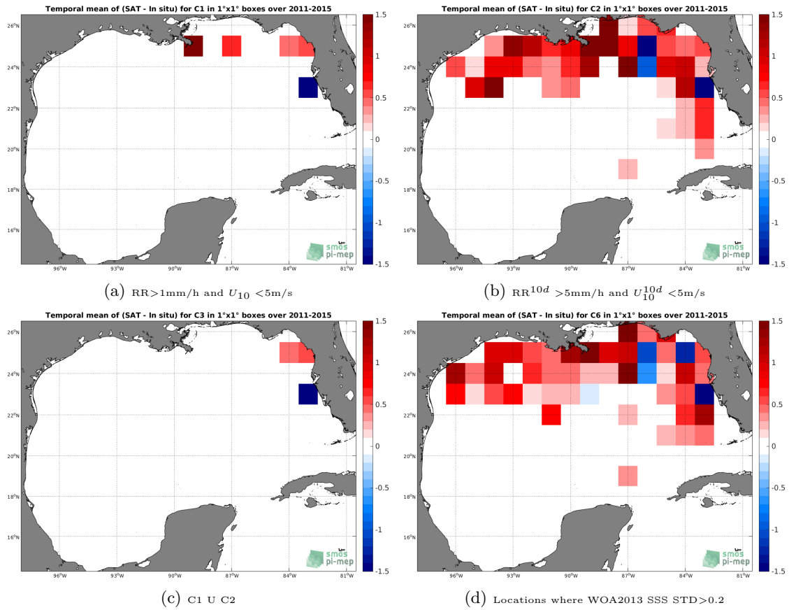
Figure 12: Temporal mean gridded over spatial boxes of size 1^\circ \times 1^\circ of \Delta SSS (Aquarius-L2-JPL-V5 - TSG-SAMOS) for 4 different subdatasets corresponding to: RR > 1\text{mm/h} and U_{10} < 5\text{m/s} (a), RR^{10d} > 5\text{mm/h} and U_{10}^{10d} < 5\text{m/s} (b), C1 U C2 (c), Locations where WOA2013 SSS STD > 0.2 (d).
