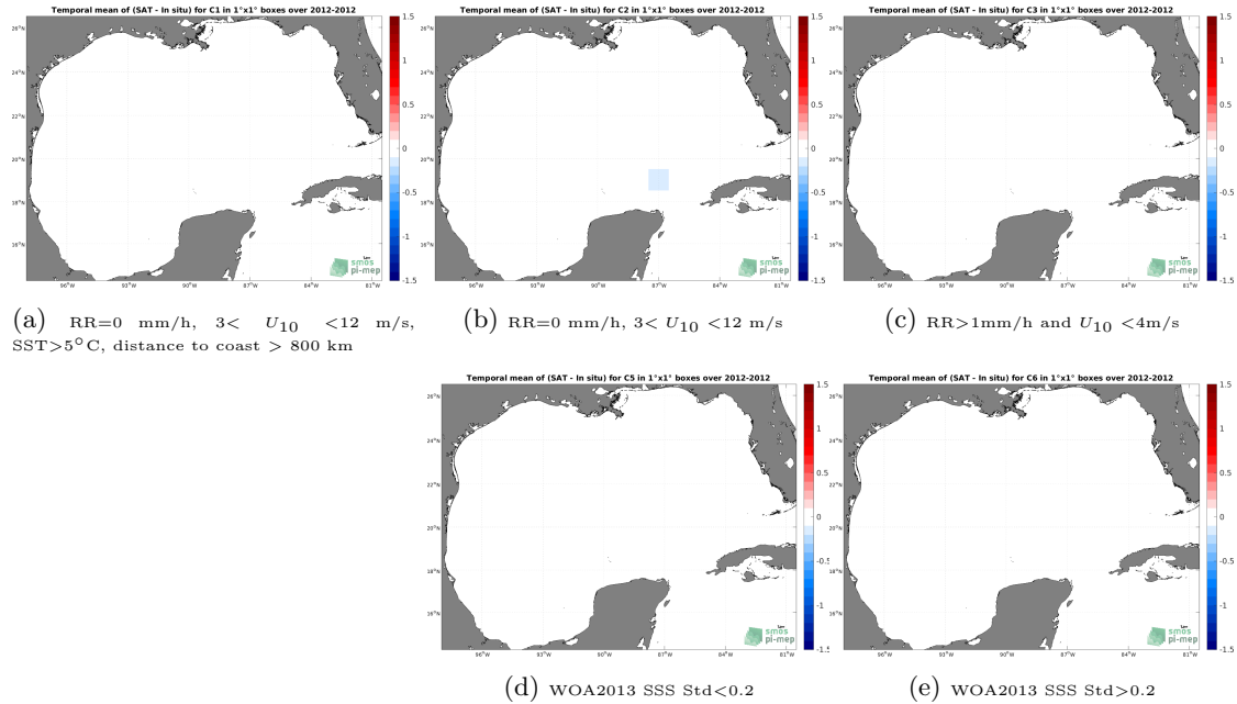
Figure 12: Temporal mean gridded over spatial boxes of size 1^{\circ}\times 1^{\circ} of \Delta SSS (Aquarius SSS L2 CAP v5 (JPL) - TSG (GOSUD-Sailing-ship)) for 5 different subdatasets corresponding to: RR=0 mm/h, 3 < U_{10} < 12 m/s, SST > 5^{\circ}\text{C} , distance to coast > 800 km (a), RR=0 mm/h, 3 < U_{10} < 12 m/s (b), RR > 1 mm/h and U_{10} < 4 m/s (c), WOA2013 SSS Std < 0.2 (d), WOA2013 SSS Std > 0.2 (e).
