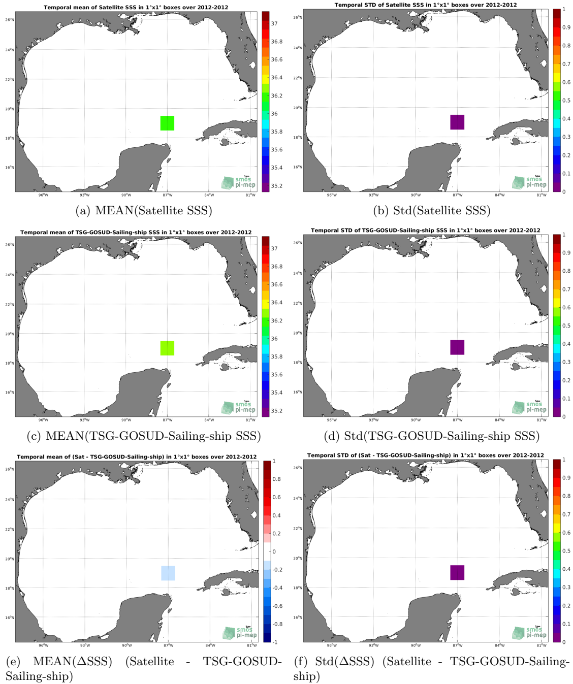
Figure 6: Temporal mean (left) and Std (right) of SSS from Aquarius-L2-JPL-V5 (top), TSG-GOSUD-Sailing-ship (middle), and of \Delta SSS (Satellite - TSG-GOSUD-Sailing-ship). Only match-up pairs are used to generate these maps.
