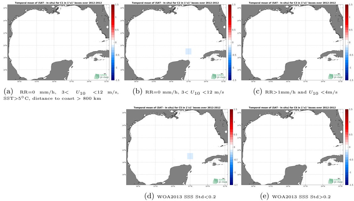
Figure 12: Temporal mean gridded over spatial boxes of size 1^\circ \times 1^\circ of \Delta SSS (Aquarius-L2-JPL-V5 - TSG-GOSUD-Sailing-ship) for 5 different subdatasets corresponding to:RR=0 mm/h, 3 < U_{10} < 12 m/s, SST >5^\circ\text{C} , distance to coast > 800 km (a), RR=0 mm/h, 3 < U_{10} < 12 m/s (b), RR >1 mm/h and U_{10} < 4 m/s (c), WOA2013 SSS Std <0.2 (d), WOA2013 SSS Std >0.2 (e).
