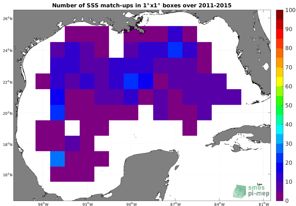
Figure 4: Number of SSS match-ups between Argo SSS and the Aquarius SSS L2 CAP v5 (JPL) SSS product for the Gulf of Mexico Pi-MEP region over 1^\circ \times 1^\circ boxes and for the full satellite product period.
