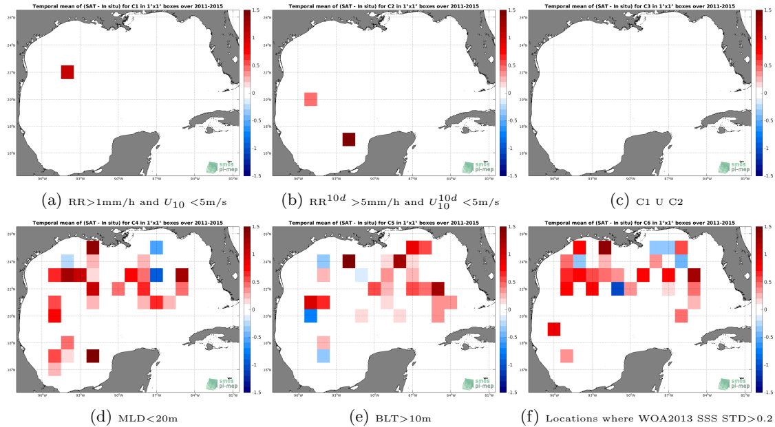
Figure 12: Temporal mean gridded over spatial boxes of size 1^\circ \times 1^\circ of \Delta\text{SSS} (Aquarius-L2-JPL-V5 - Argo) for 6 different subdatasets corresponding to: RR > 1\text{mm/h} and U_{10} < 5\text{m/s} (a), RR^{10d} > 5\text{mm/h} and U_{10}^{10d} < 5\text{m/s} (b), C1 U C2 (c), MLD < 20\text{m} (d), BLT > 10\text{m} (e), Locations where WOA2013 SSS STD > 0.2 (f).
