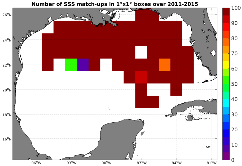
Figure 4: Number of SSS match-ups between TSG-SAMOS SSS and the AQUARIUS-L2-JPL-V4 SSS product for the Gulf of Mexico Pi-MEP region over 1^\circ \times 1^\circ boxes and for the full satellite product period.
