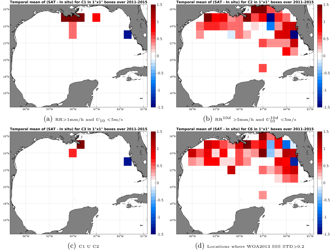
Figure 12: Temporal mean gridded over spatial boxes of size 1^\circ \times 1^\circ of \Delta SSS (AQUARIUS-L2-JPL-V4 - TSG-SAMOS) for 4 different subdatasets corresponding to: RR > 1 mm/h and U_{10} < 5 m/s (a), RR 10d > 5 mm/h and U_{10}^{10d} < 5 m/s (b), C1 U C2 (c), Locations where WOA2013 SSS STD > 0.2 (d).
