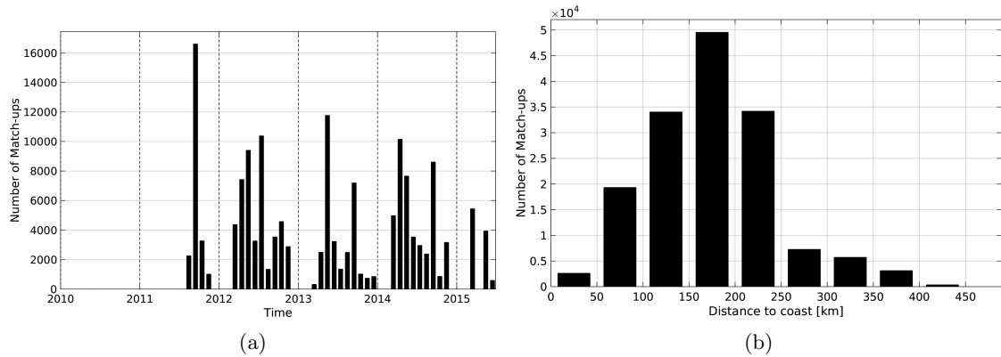
Figure 1: Number of match-ups between TSG-SAMOS and AQUARIUS-L2-JPL-V4 SSS as a function of time (a) and as function of the distance to coast (b) over the Gulf of Mexico Pi-MEP region and for the full satellite product period.
