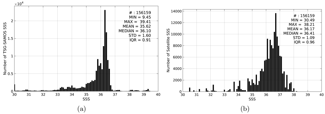
Figure 2: Histograms of SSS from TSG-SAMOS (a) and AQUARIUS-L2-JPL-V4 (b) considering all match-up pairs per bins of 0.1 over the Gulf of Mexico Pi-MEP region and for the full satellite product period.
